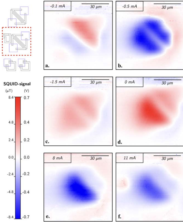
Figure 7. SSM-scans of a pair of triangular \pi -loops with 3 \mu\text{m} ds -JJs. Area: 75 \mu\text{m} \times 75 \mu\text{m} , resolution: 75 \text{ px} \times 75 \text{ px} , scanning speed: 50 \mu\text{m s}^{-1} , 3-point levelled. On the top left, the mask design of the scanning area is illustrated. The induction currents are indicated in the top left corners of the scans. The color scale at the bottom left represents the SQUID voltage and the corresponding local amplitude of the B_z component of the magnetic field.
