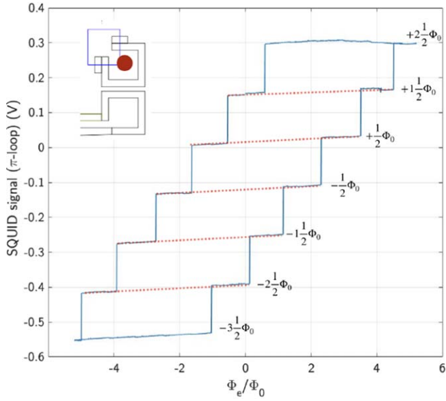
Figure 9. Hysteresis loop of a square \pi -loop with 6 \mu\text{m} ds -JJs measured by the SSM as a function of applied magnetic flux. The bias flux was subtracted from the SQUID signal. Insert shows the mask design of the related part of the sample with the location of the SQUID sensor (not to scale) circled.
