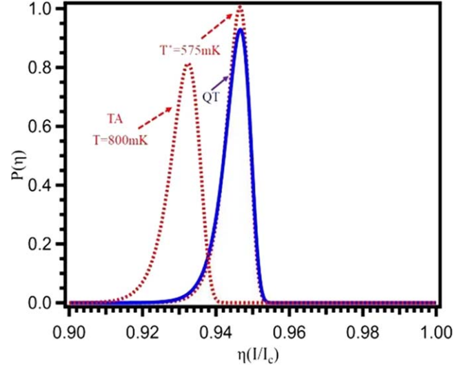
Figure 15. Theoretical estimations of transition temperature from thermal activation (TA) to quantum tunneling (QT) modes for hypothetical YBCO–MoRe ds -JJs that have junction area 200 \text{ nm} \times 200 \text{ nm} .
