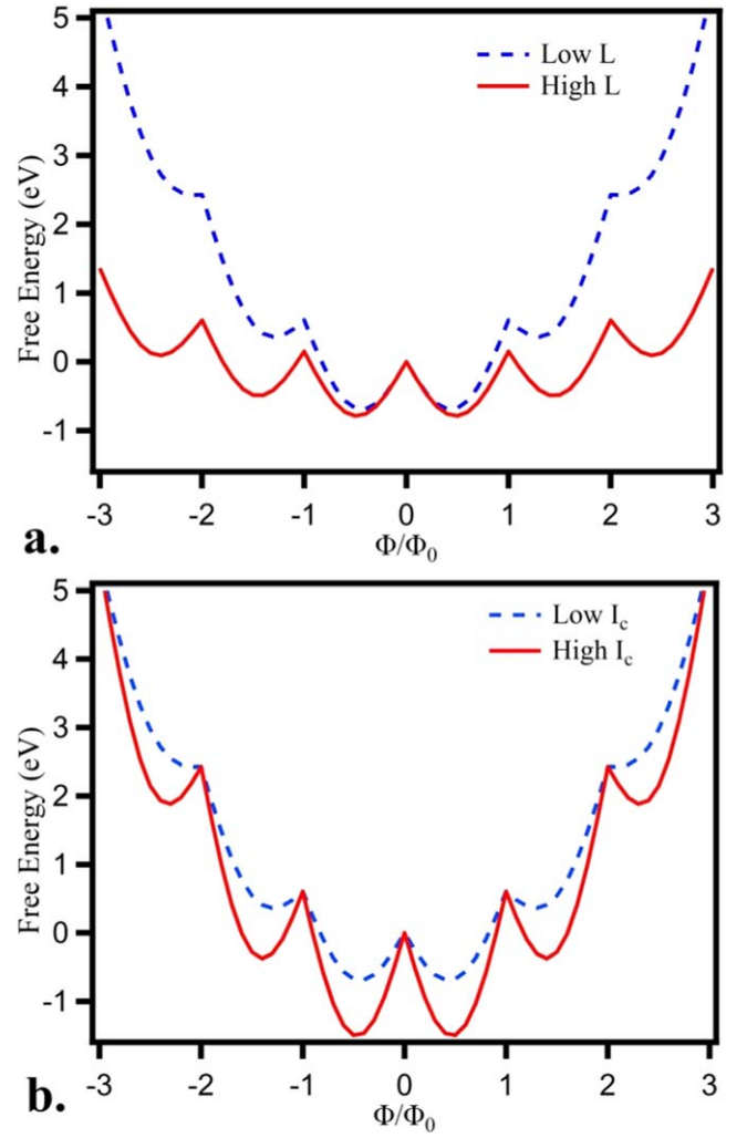
Figure 10. Theoretical dependences of free energy U of \pi -loops that have equal critical currents I_{c1} = I_{c2} of the ds -JJs in the case of \Phi_e = 0 with variations in the (a) inductance and (b) critical current. The magnetic flux in the \pi -loops \Phi is normalized in units of \Phi_0 .
