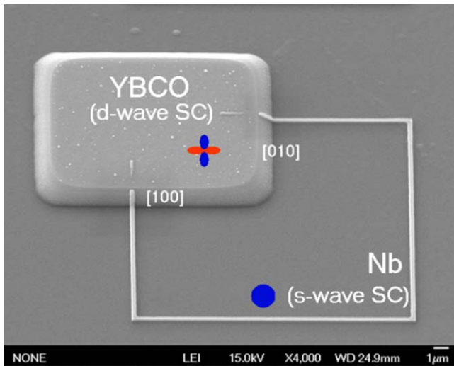
Figure 14. SEM image of a \pi -loop with 200 \text{ nm} \times 700 \text{ nm} YBCO–Nb ds -JJs produced with the help of an e-beam lithography.
