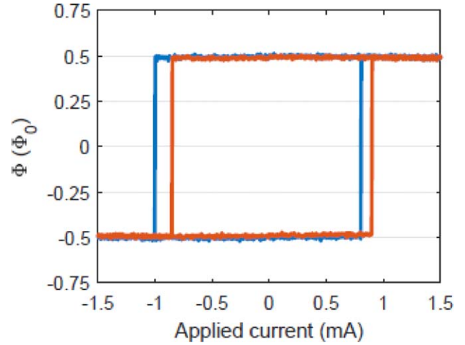
Figure 8. Comparison between two sweeps with the loop ‘II’ in different states.
