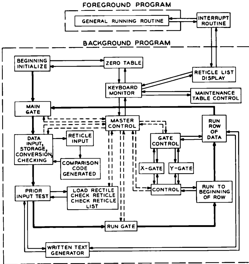
Fig. 19—Program block flow diagram.
