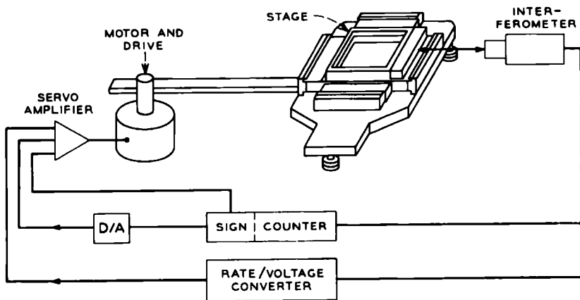
Fig. 16—Block diagram of stage-positioning servo system.
