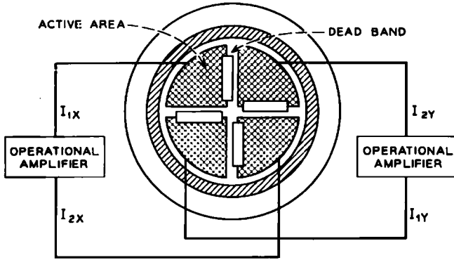
Fig. 7—Photo diode.
