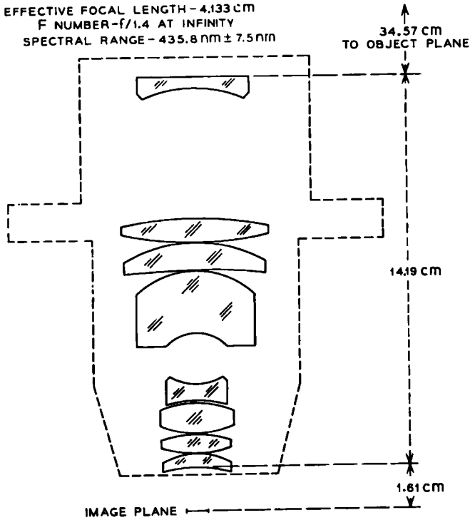
Fig. 4—Projection lens.
