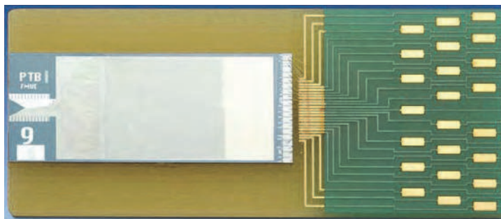
Fig. 5. Photo of a 10 V programmable Josephson junction series array.
