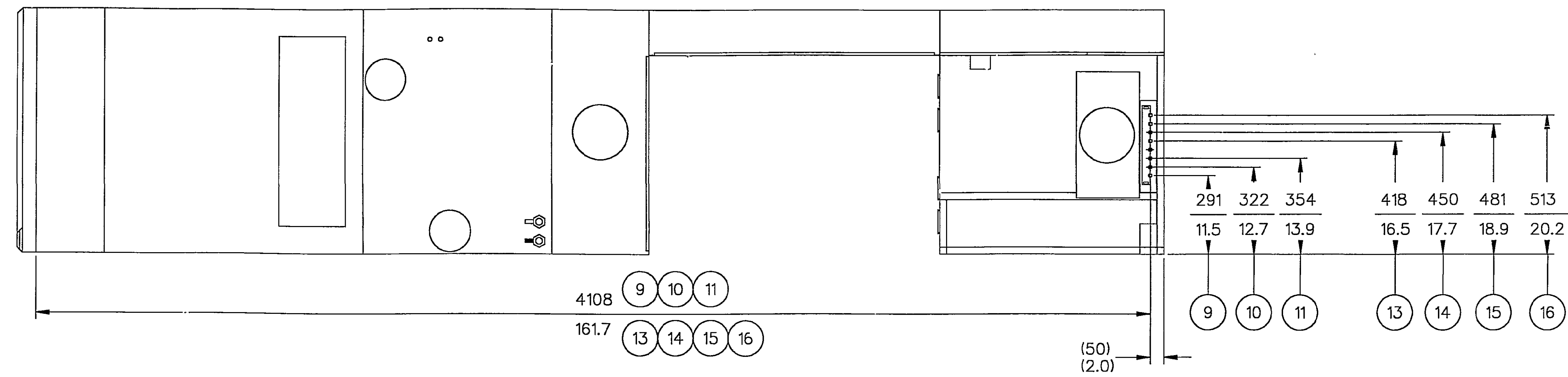
VIEW F-F
