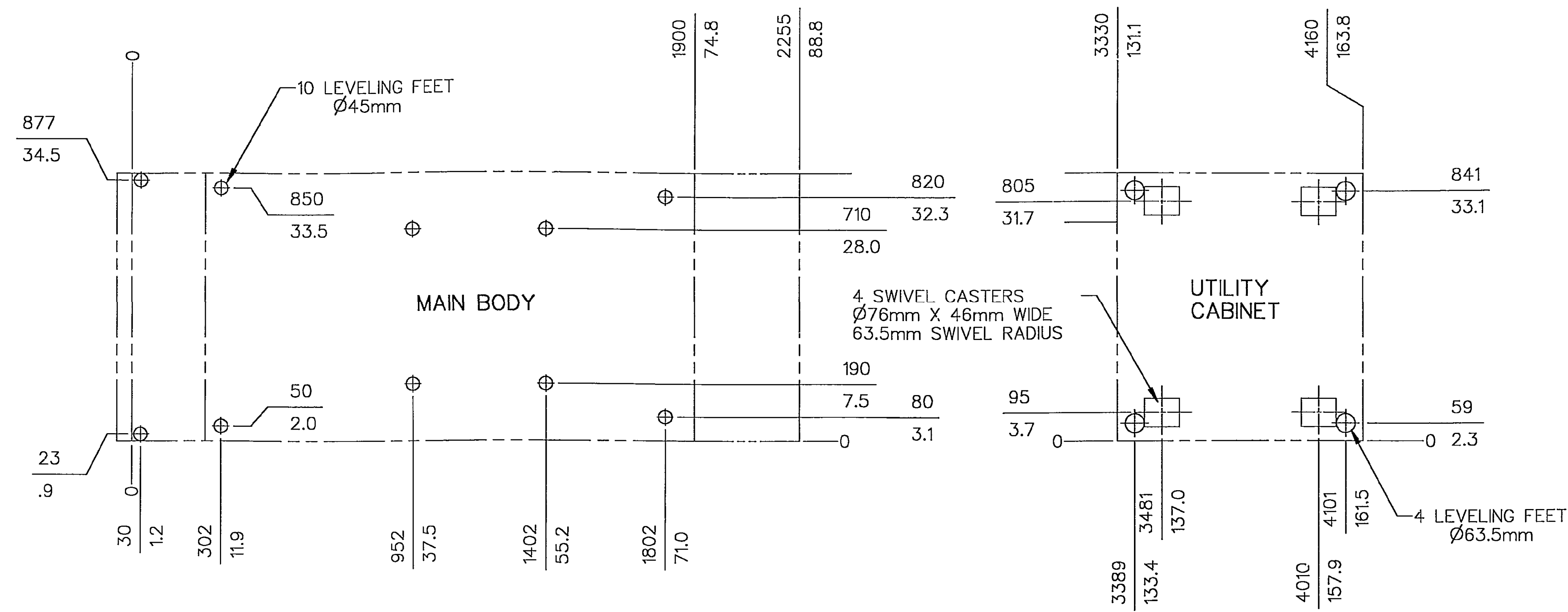
TOP VIEW - LEVELING FEET/CASTER LOCATION
