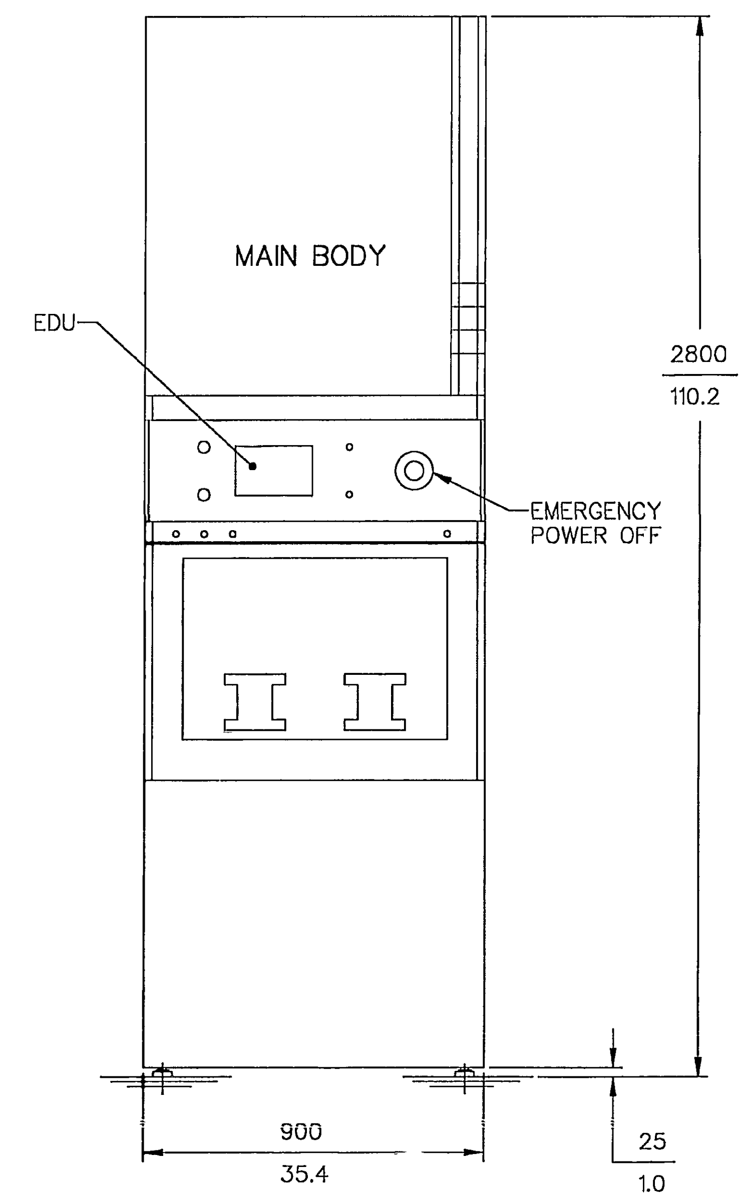
VIEW D-D
