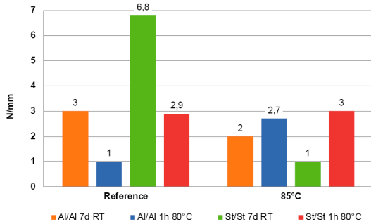
Floating roller peel resistance, DELO standard 38
