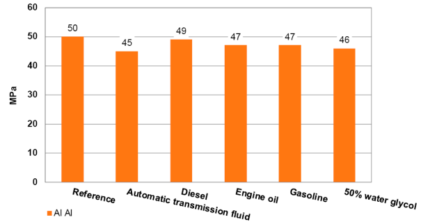
Compression shear strength after media storage for 1000 h, DELO Standard 5 curing: 1h +80°C
