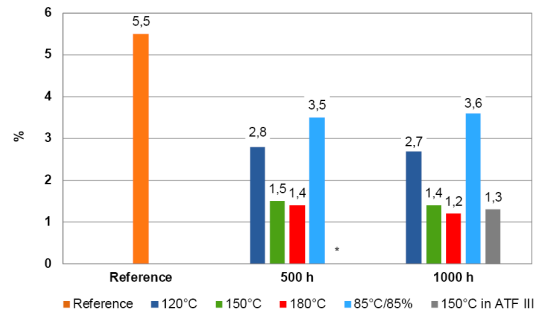
Elongation at tear after temperature storage, by the criteria of DIN EN ISO 527 Curing: 1h +80°C
