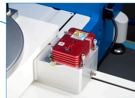
Integrated debris removal station cleans shear and pull tools automatically between tests
