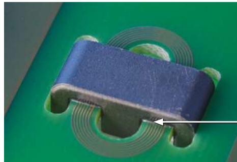
Bonding ferrite elements to an FR4 PCB
