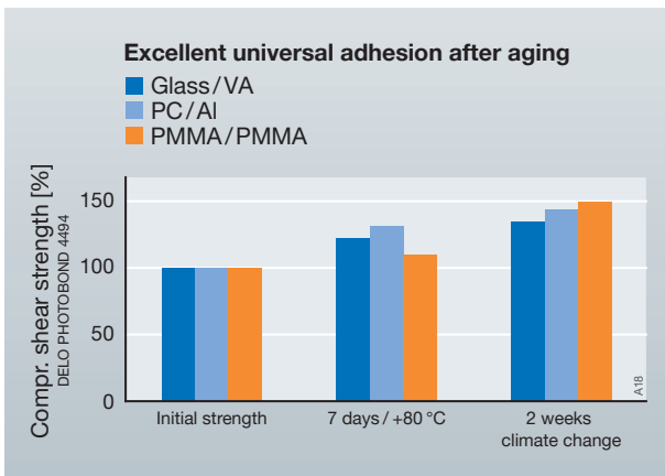
During the aging process compression shear strength increases slightly while at the same time tension-equalizing properties are preserved.
