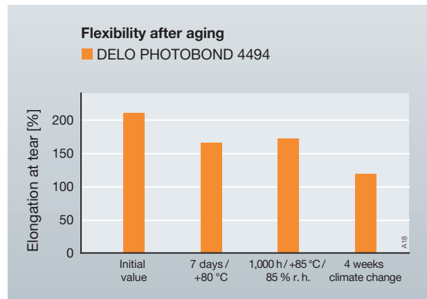
Even after the aging process DELO PHOTOBOND 4494 retains its flexibility with elongation at tear greater than 120%.
