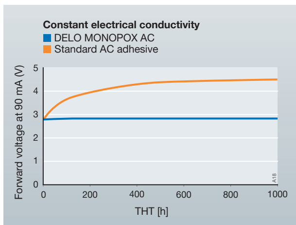
DELO MONOPOX AC adhesives ensure constant electrical conductivity.
