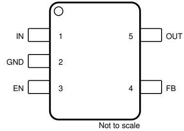
Figure 4-2. DBV Package, 5-Pin Adjustable SOT-23 (Top View)
