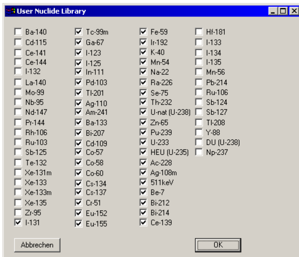
Figure 47 winTMCA32 nuclide library for identification
