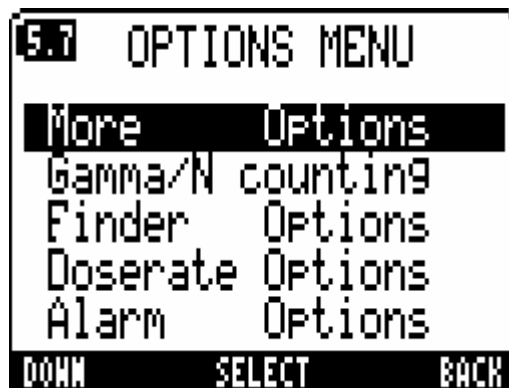
Figure 17 Options menu
