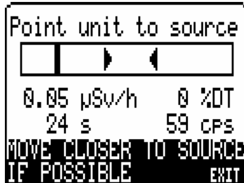
Figure 13 Starting screen for the IDENT mode
