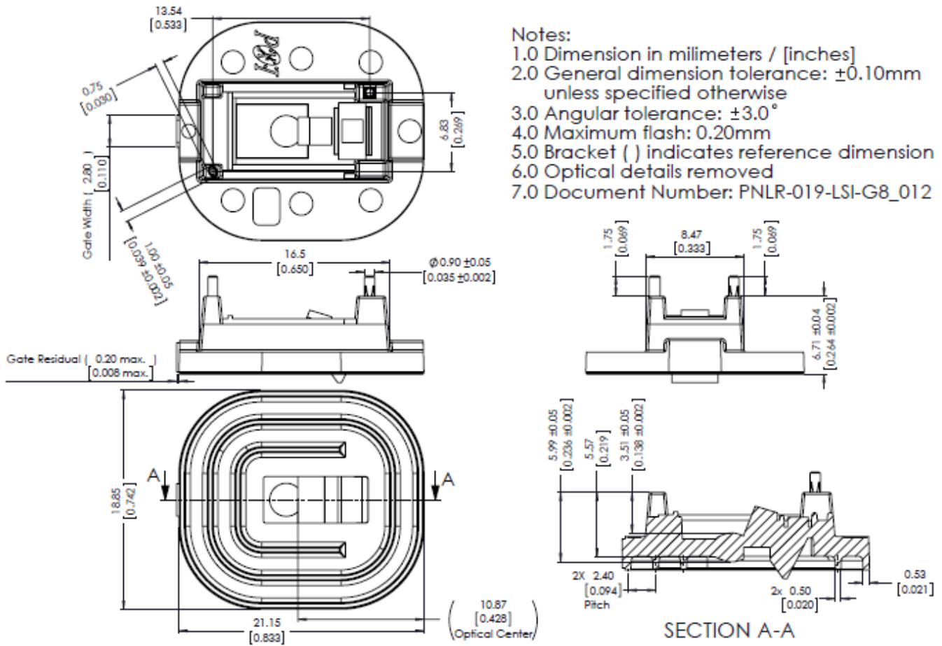
Figure 7. LM19-LSI Lens Outline Drawing
