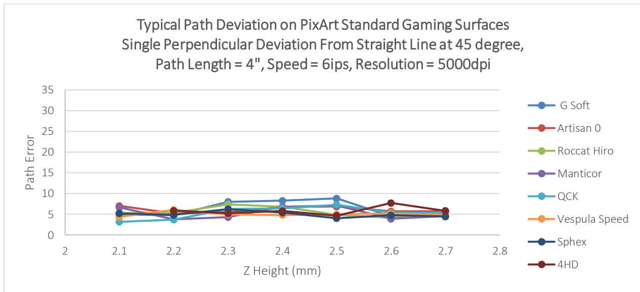
Figure 12. Path Error vs. Z Height at resolution of 5000dpi
