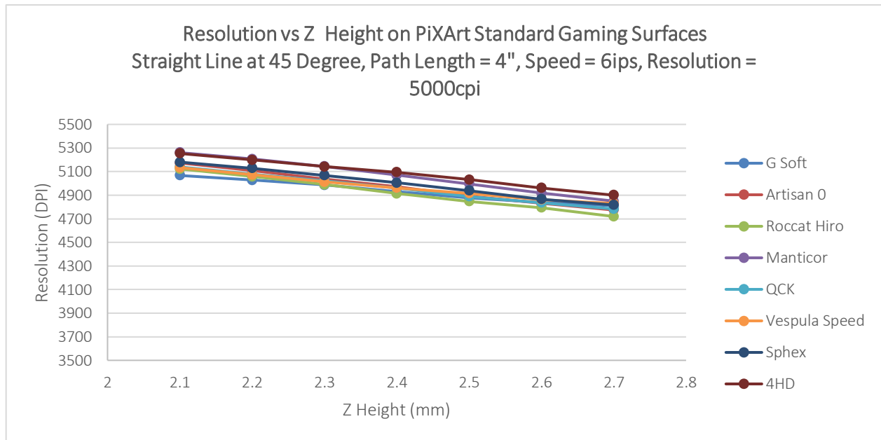
Figure 11. Mean Resolution vs. Z Height at resolution of 5000dpi
