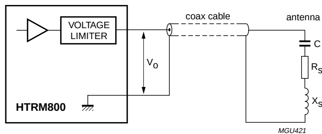
Fig.6 Basics of the long range antenna.
