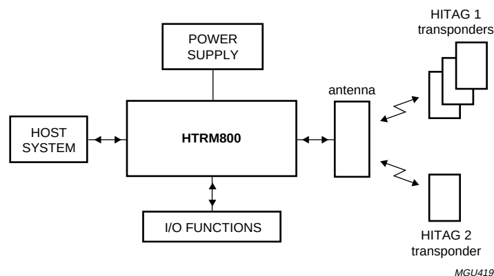
Fig.3 System overview.
