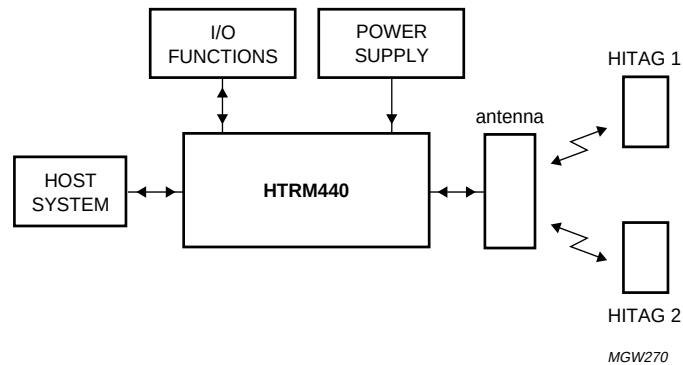
Fig.5 System overview.
