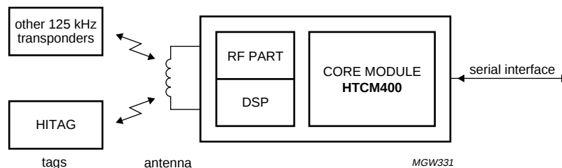
Fig.11 Block diagram of long range reader module.
