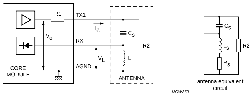
Fig.12 Architecture of a proximity antenna.
