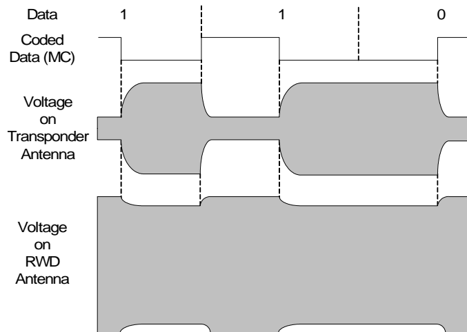
Fig.5 Data Transmission Transponder to Read/Write Device.
