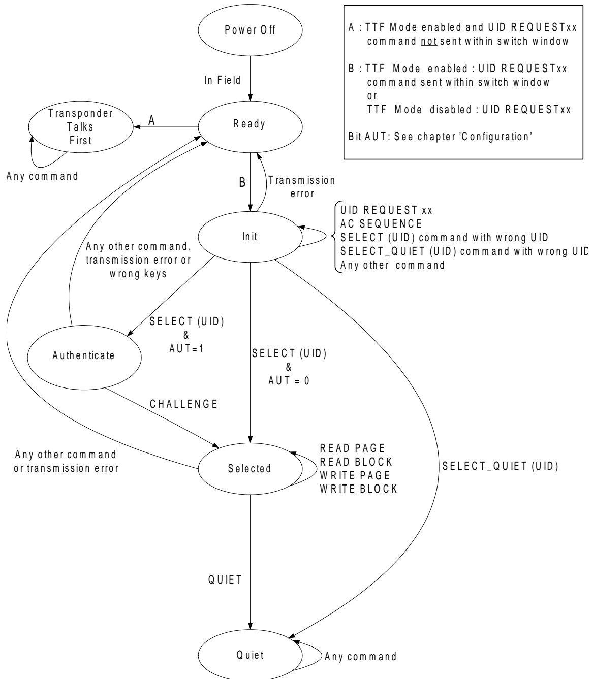
Fig.17 State diagram HITAG S 256 and HITAG S 2048.
