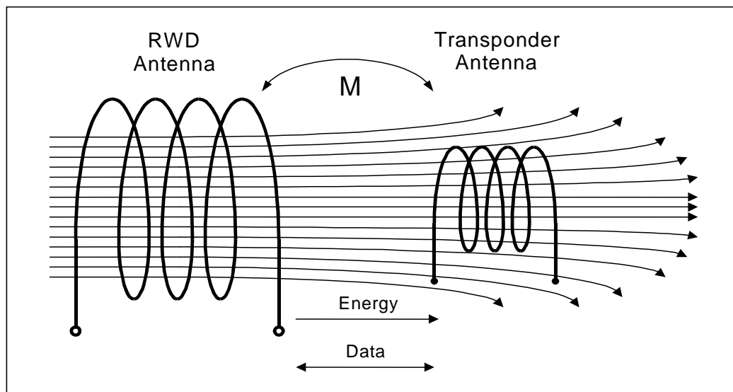
Fig.4 Loose coupled transformer.
