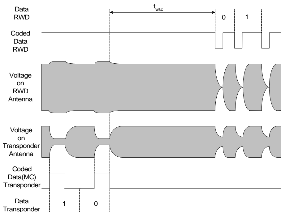
Fig.10 Read/Write Device waiting time before sending a subsequent command.
