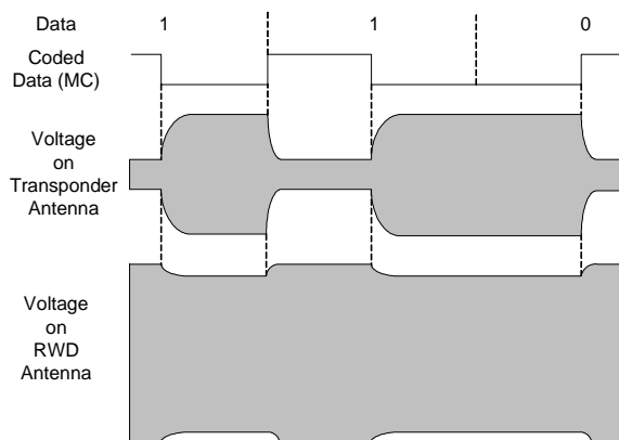
Fig.5 Data Transmission Transponder to Read/Write Device.
