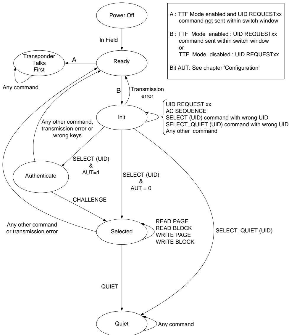
Fig.17 State diagram HITAG S 256 and HITAG S 2048.
