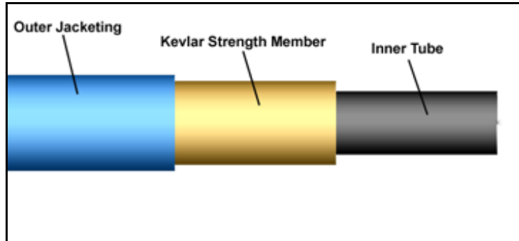
Figure 2: Typical Jacketed Fiber Construction
