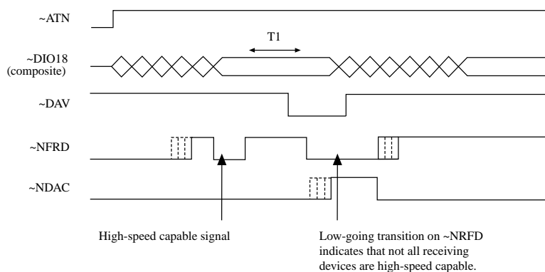
Figure 18. HS488-Capable Talker
