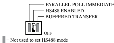
Figure 10. DIP Switch Setting for Enabled HS488
