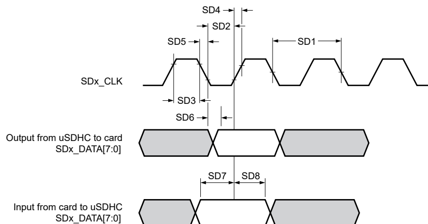
Figure 58. SD/eMMC4.3 High Speed Mode Interface Timing
