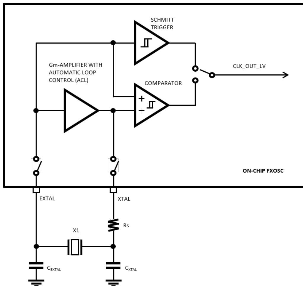
Figure 39. Block diagram
