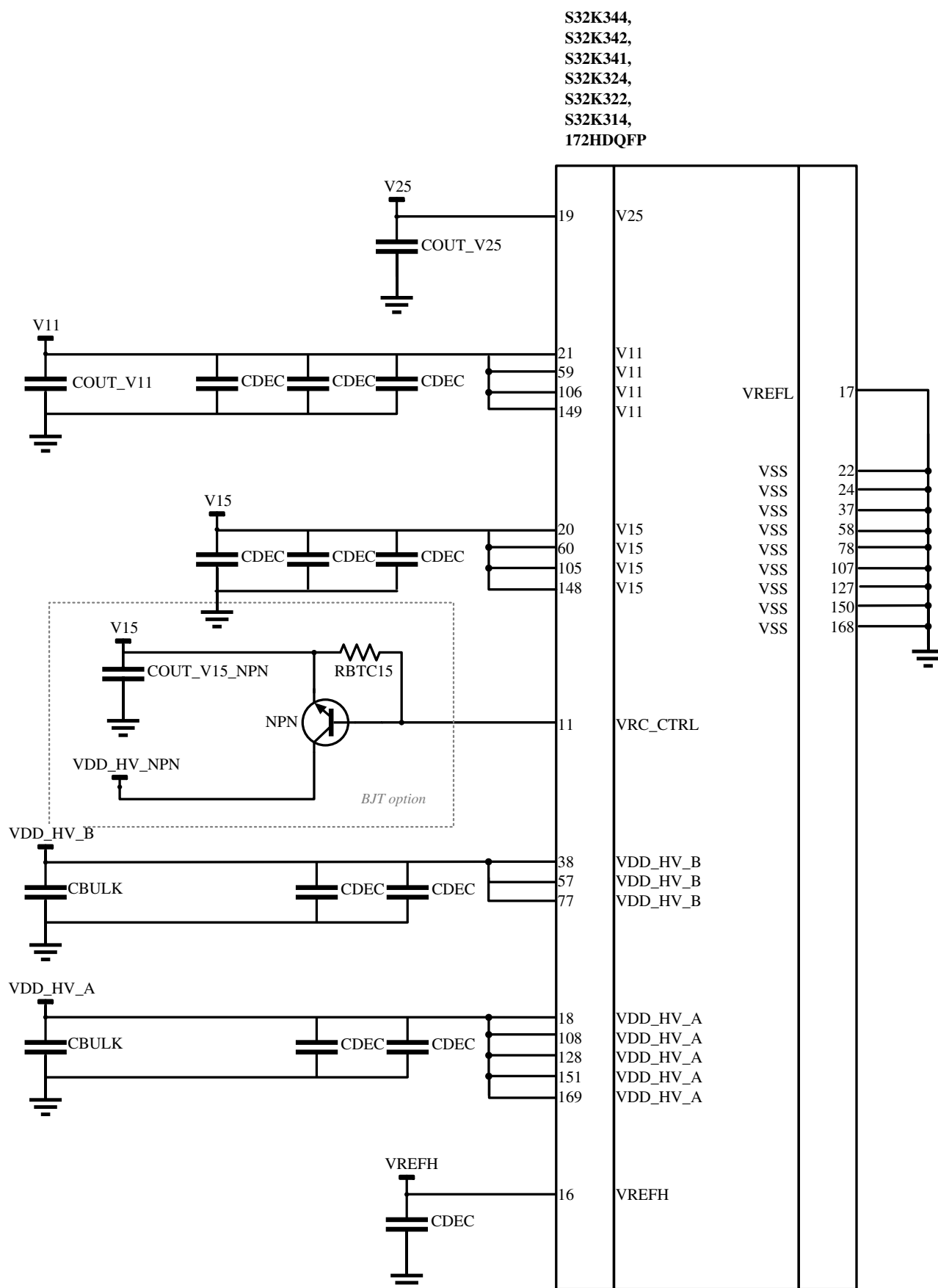
Figure 20. 172-pin HDQFP decoupling capacitor pinout diagram (S32K344, S32K324, S32K314, S32K342, S32K341 and S32K322)
