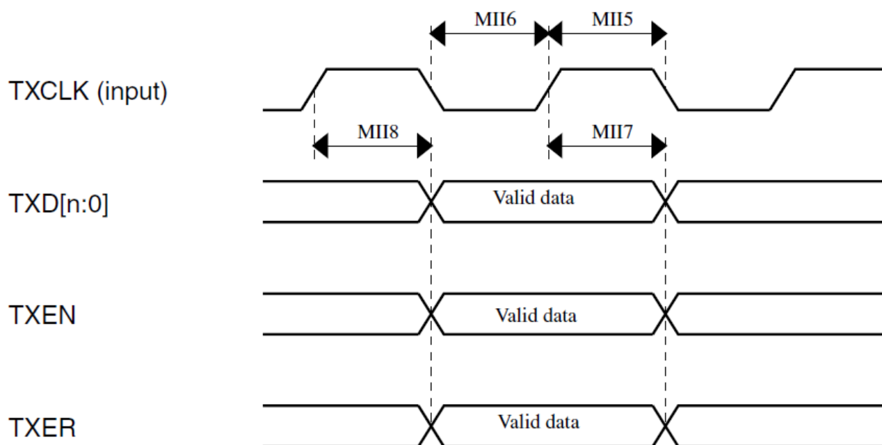
Figure 50. MII transmit diagram
