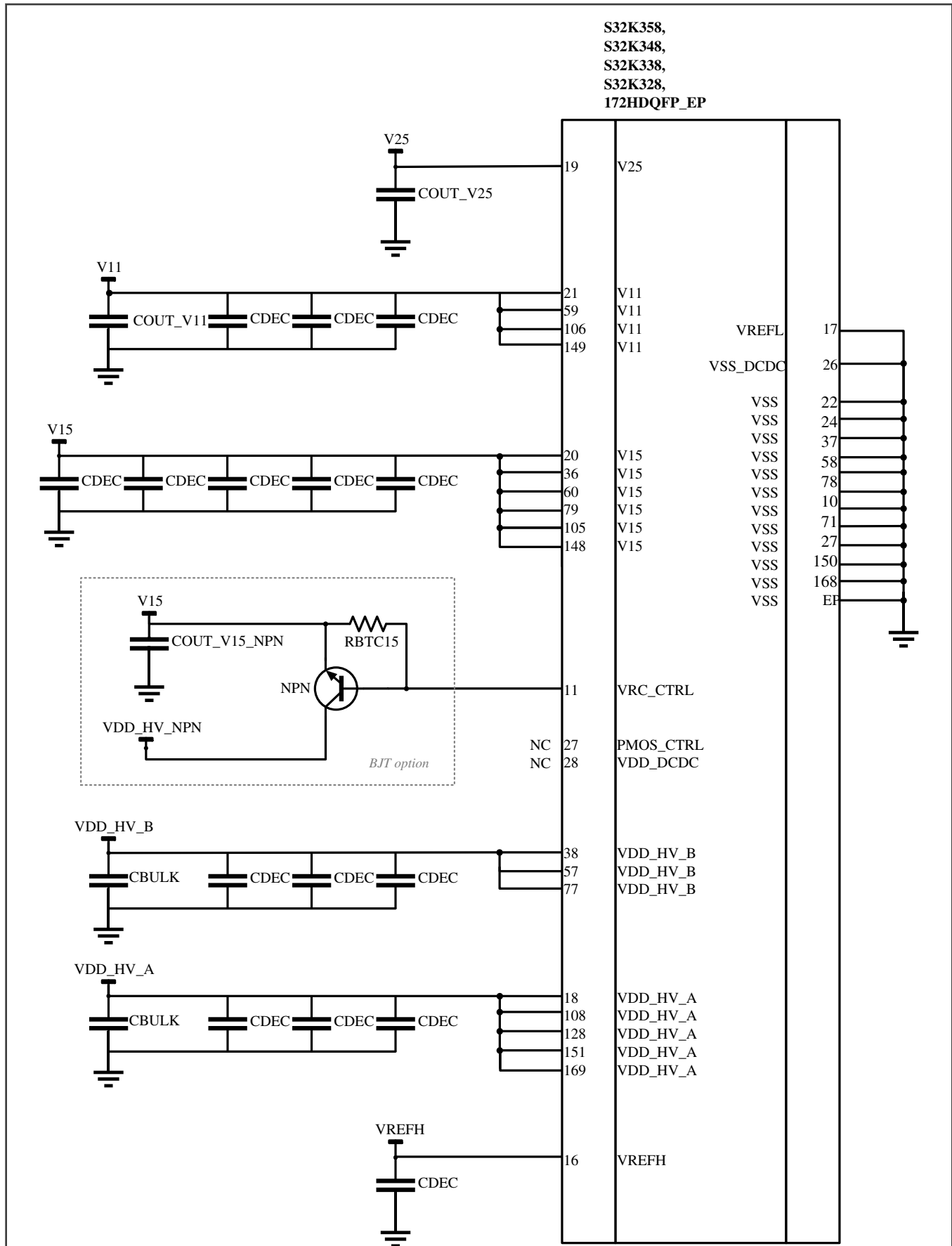
Figure 22. 172-pin HDQFP decoupling capacitor pinout diagram (S32K358, S32K348, S32K338 and S32K328)
