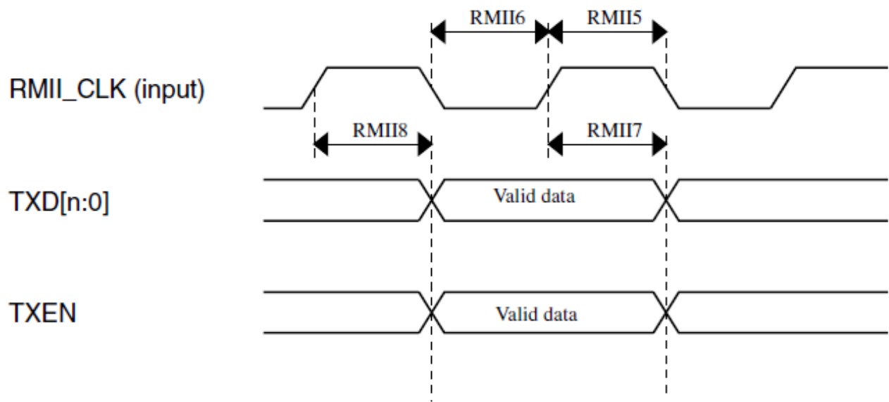
Figure 52. RMI transmit diagram
