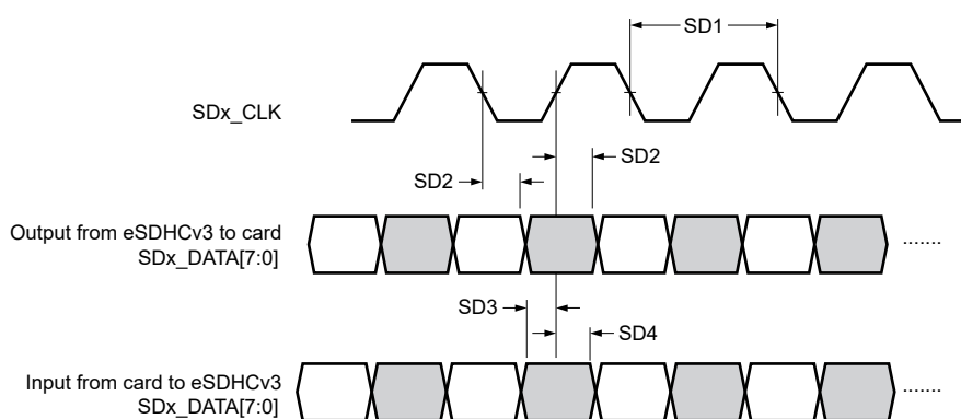
Figure 59. SD/eMMC4.4/4.41 DDR50 Mode Interface Timing
