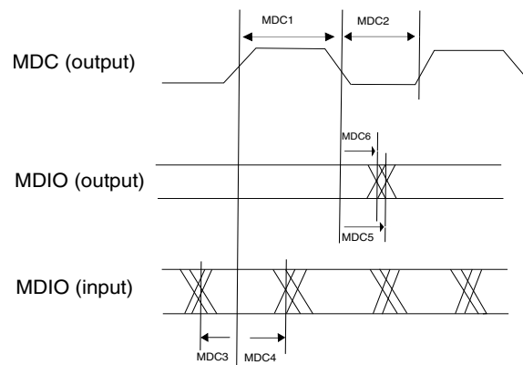
Figure 55. MII/RMII serial management channel timing
