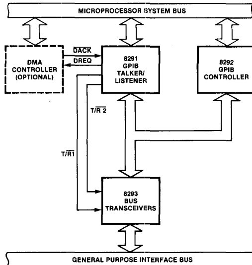
Figure 1. 8291, 8292 Block Diagram
