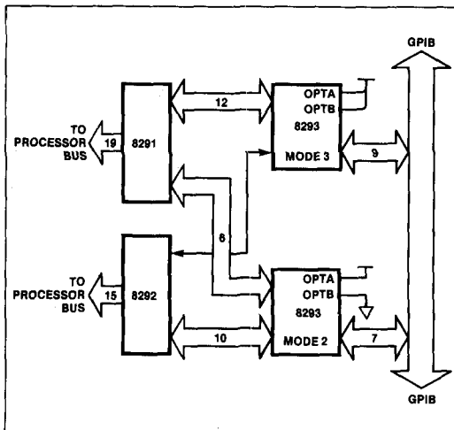
Figure 3. Talker/Listener/Controller Configuration
