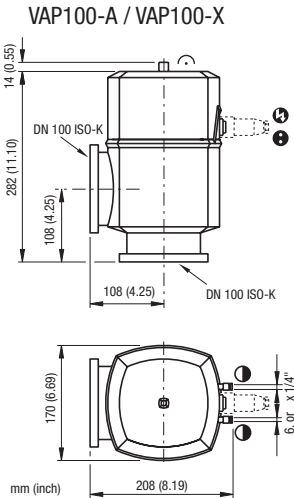
Angle valve with and without pilot valve, with position indicator
