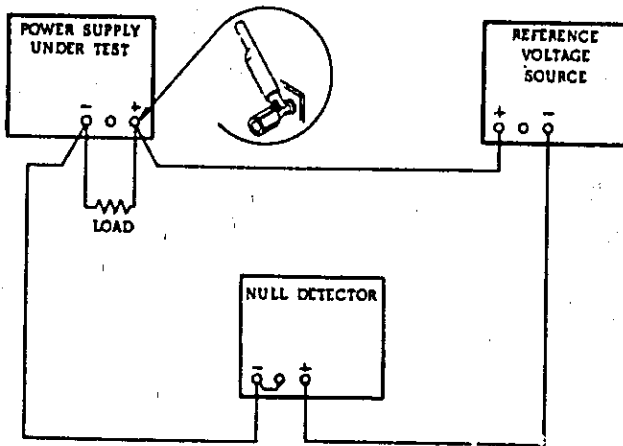
Figure 5-3. Differential Voltmeter Substitute Test Setup
