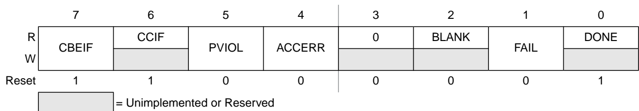
Figure 1-10. EEPROM Status Register (ESTAT - Special Mode)
