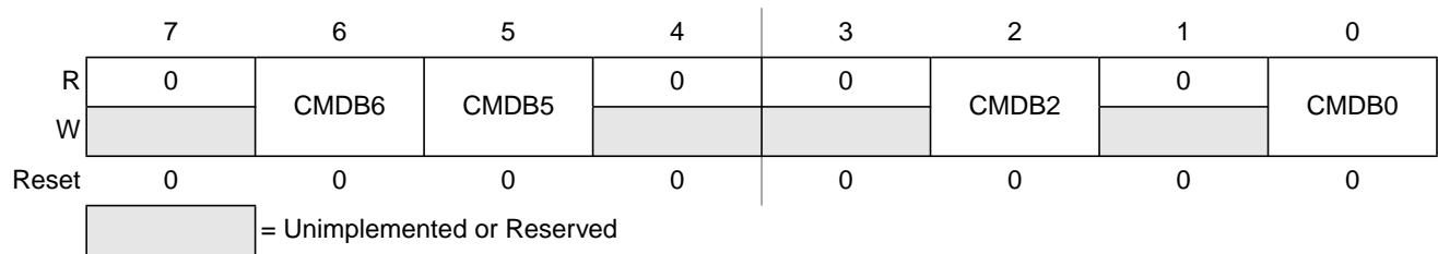
Figure 1-11. EEPROM Command Register (ECMD)
