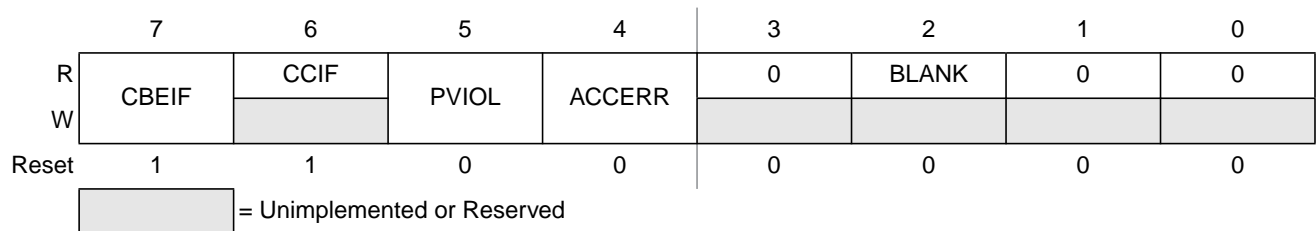
Figure 1-9. EEPROM Status Register (ESTAT - Normal Mode)
