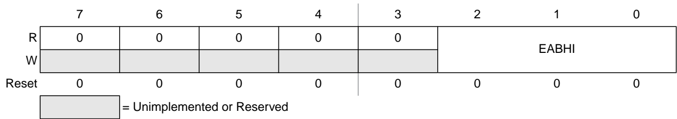
Figure 1-13. EEPROM Address High Register (EADDRHI)
