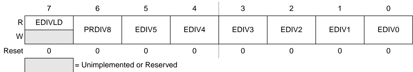
Figure 1-4. EEPROM Clock Divider Register (ECLKDIV)
