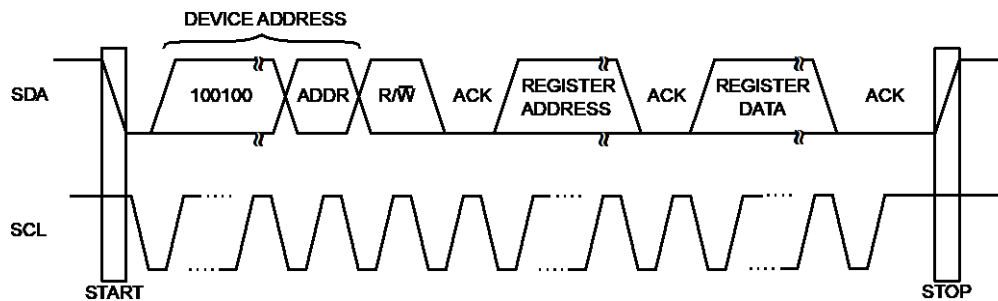
Figure 14 - I 2 C Slave Interface
