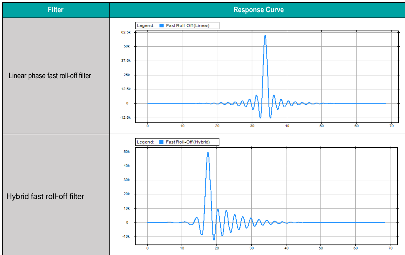
Figure 10 - PCM Filter Impulse Response
