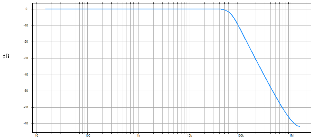
Figure 11 - DSD Filter Characteristics
