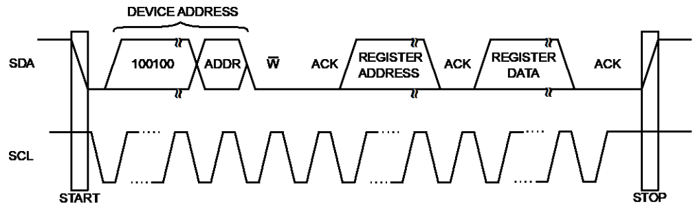
Figure 15 - I 2 C Synchronous Slave Interface
