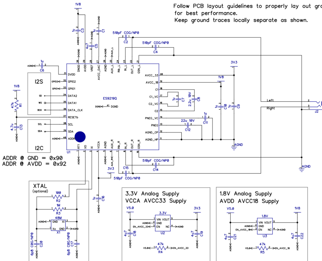
Figure 22 - ES9219MQ, ES9219Q Reference Schematic
