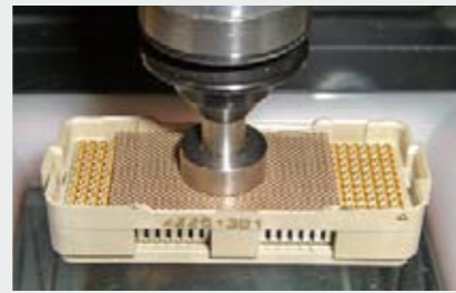
BGA Plastic Socket
