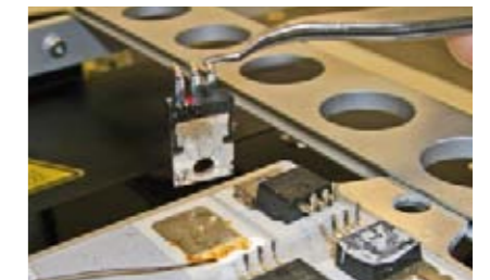
TO220 on Aluminium Carrier with HYBRID
