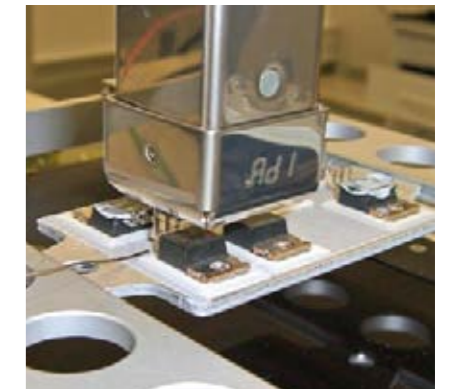
TO220 on Aluminium Carrier with HYBRID
