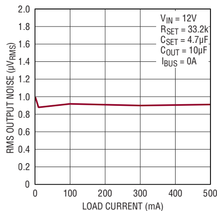
RMS Noise vs I OUT
