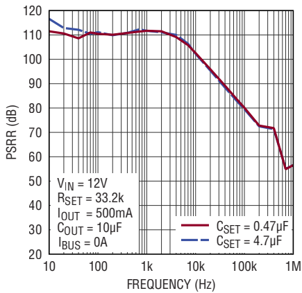
PSRR vs C SET
