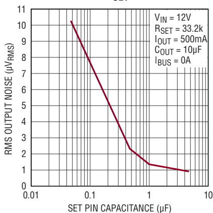
RMS Noise vs C SET
