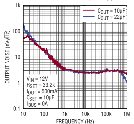
Noise Spectral Density vs C OUT
