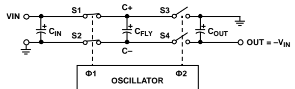
Figure 41. Basic Inverting Charge Pump
