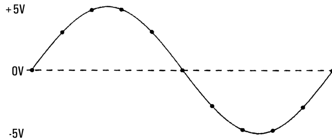
Figure 26. Level triggering at zero crossing, positive slope
