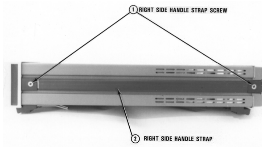
Figure 35. 3458 Right side
