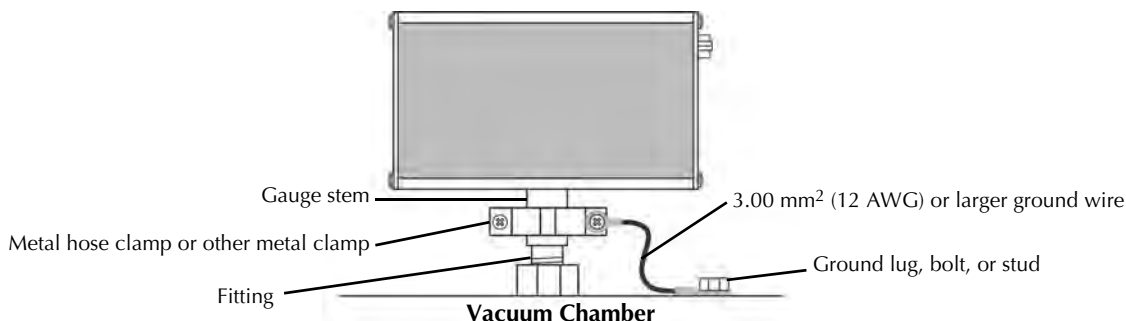
Figure 2-7 Ground Connection to the Vacuum Chamber
