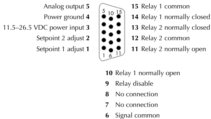
Figure 2-5 15-Pin Connector for Module with two Setpoint Relays
