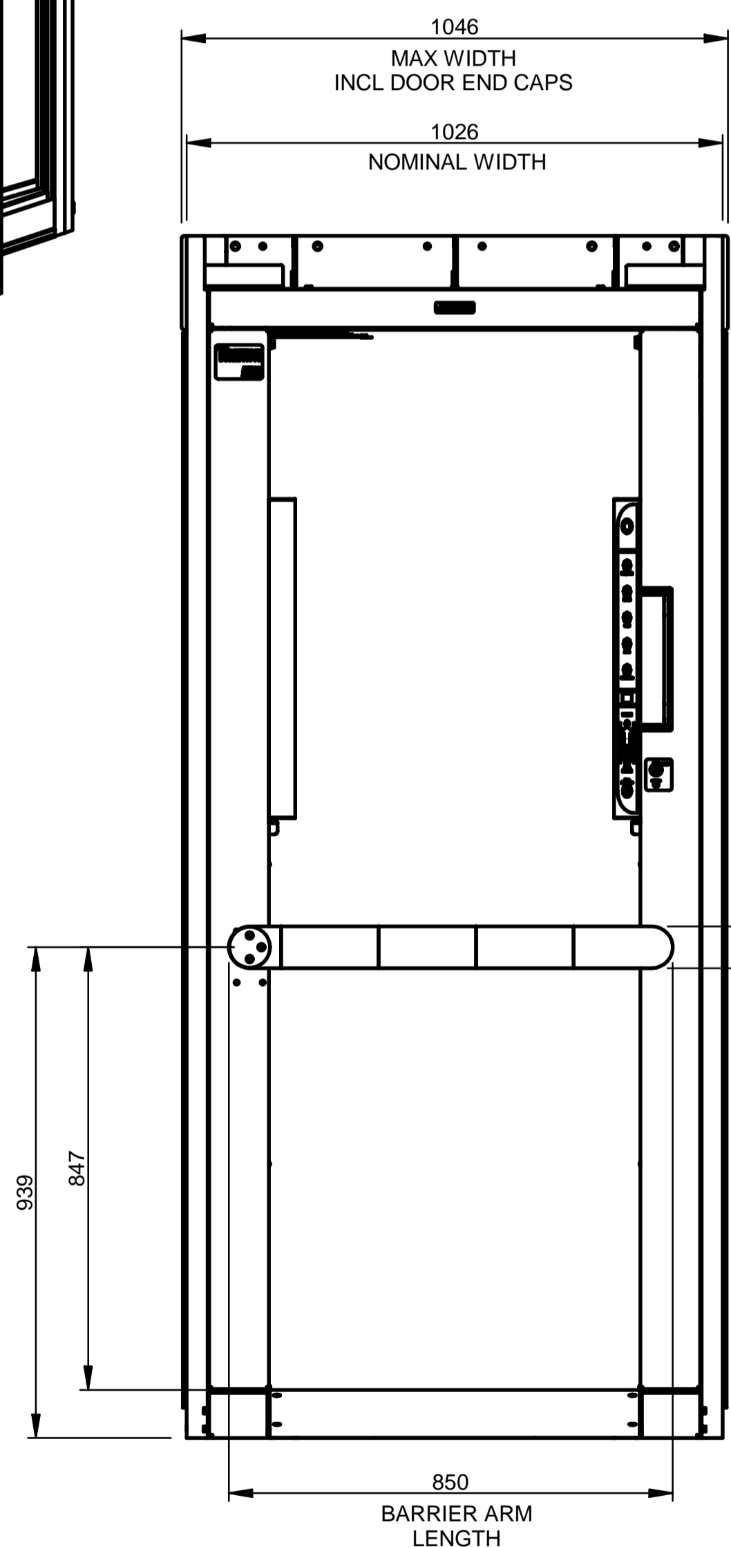
BARRIER ARM ENTRANCE VIEW (DOORS FULLY OPEN)
