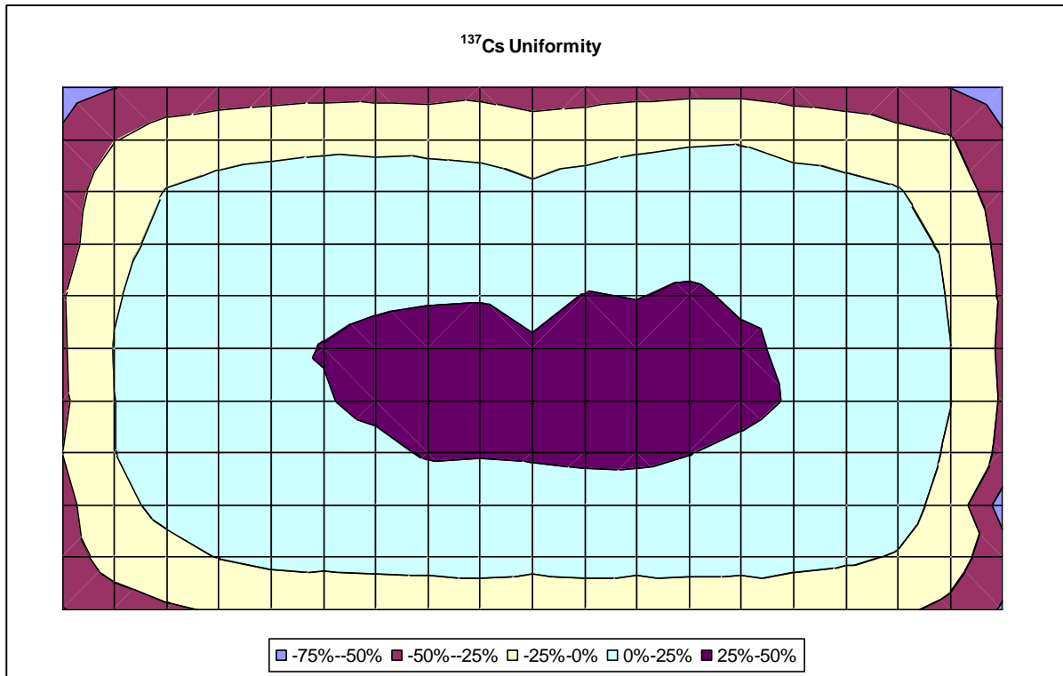
Figure 6 Foot detector uniformity to 137Cs
