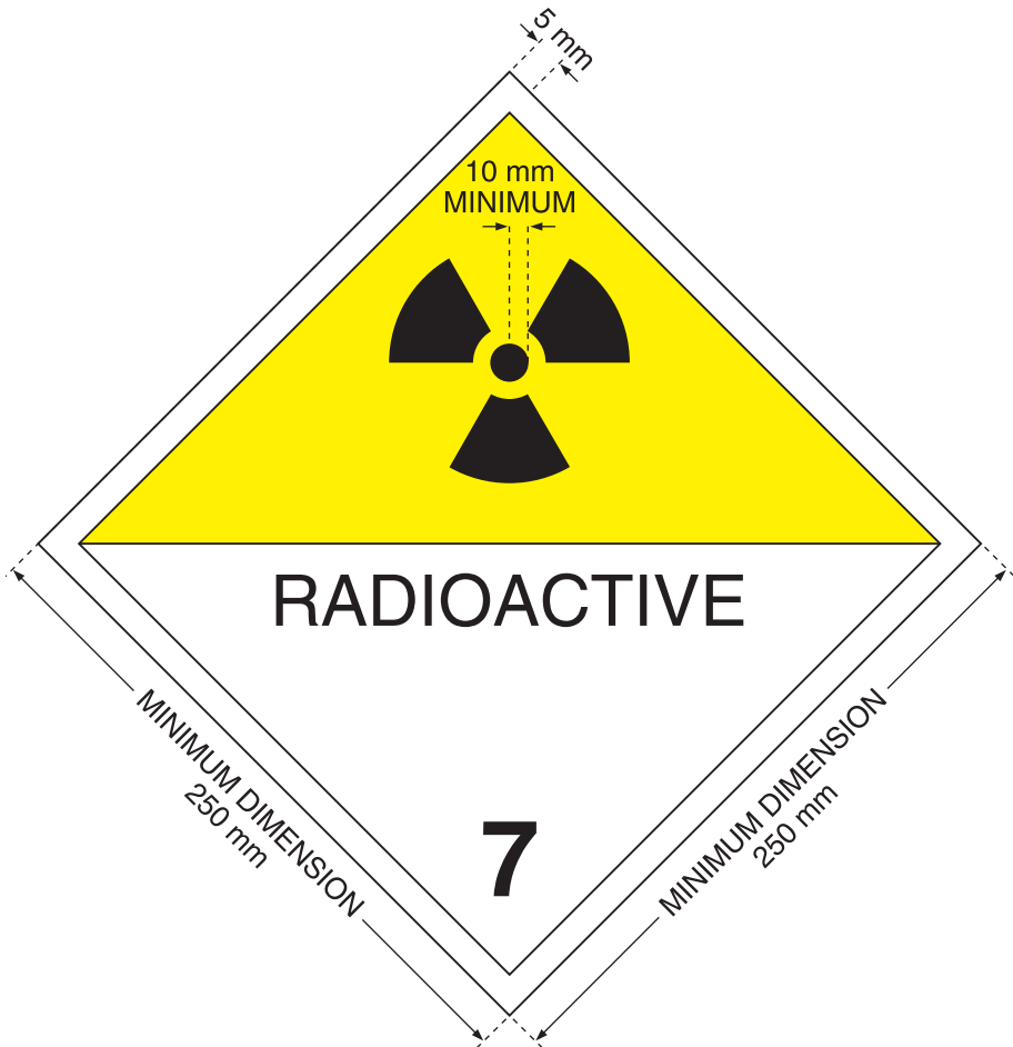
FIG. 6. Placard. Except as permitted by para. 567, minimum dimensions shall be as shown; when different dimensions are used, the relative proportions must be maintained. The number “7” shall not be less than 25 mm high. The background colour of the upper half of the placard shall be yellow and of the lower half white, the colour of the trefoil and the printing shall be black. The use of the word “RADIOACTIVE” in the bottom half is optional, to allow the alternative use of this placard to display the appropriate UN number for the consignment.
