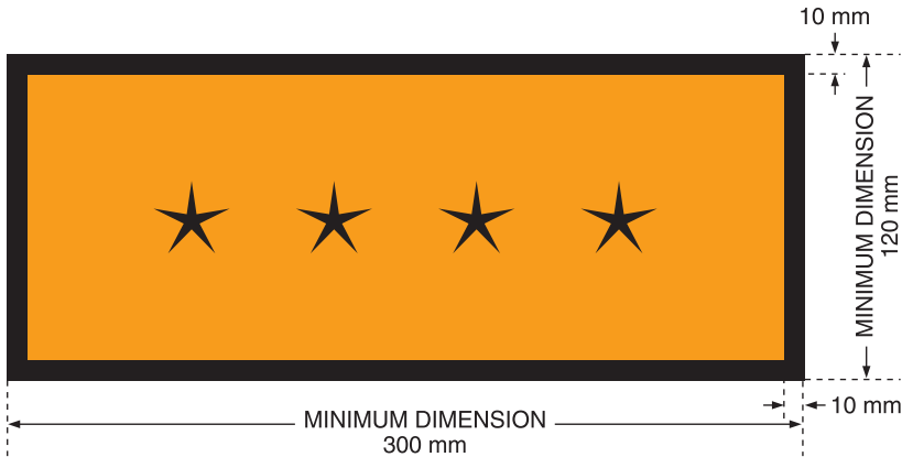
FIG. 7. Placard for separate display of UN number. The background colour of the placard shall be orange and the border and UN number shall be black. The symbol “*****” denotes the space in which the appropriate UN number for radioactive material, as specified in Table 1, shall be displayed.
