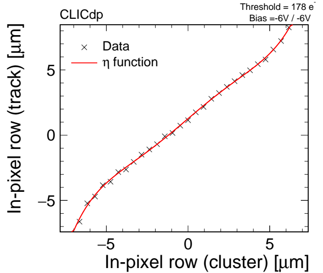
Figure 3: In-pixel telescope track position as a function of reconstructed in-pixel cluster position for the pixel flavour with segmented n-implant at a threshold of 178 e - . The 5th order polynomial fitted to the distribution (shown as red line) is defined as \eta -function.
