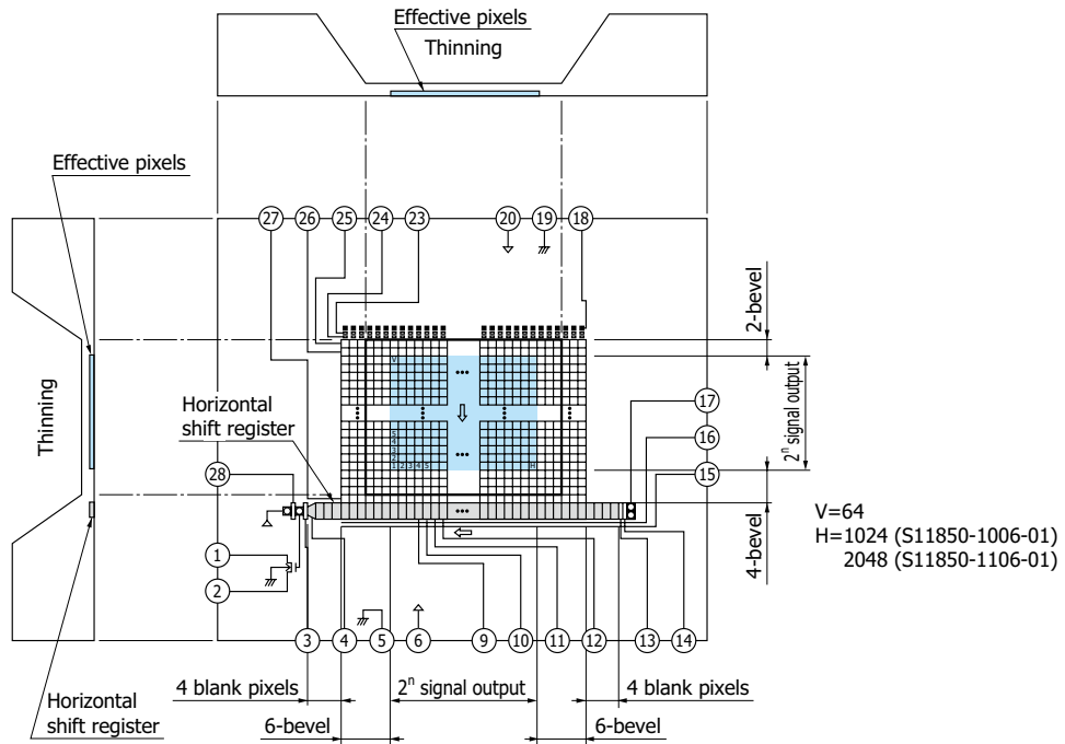
S11850-1006-01, S11850-1106-01
