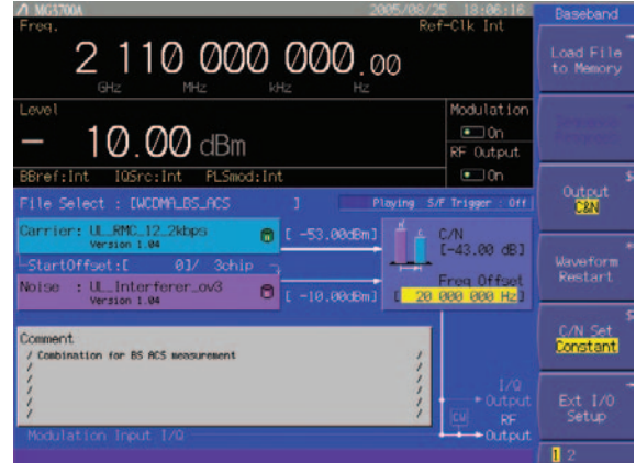
Wanted Signal + Interfering Screen
