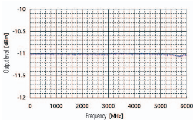
Frequency characteristic
