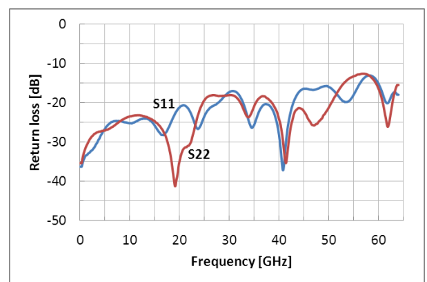
Reflection characteristics
