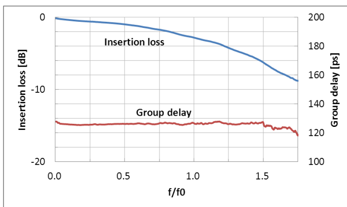
Transmission characteristic
