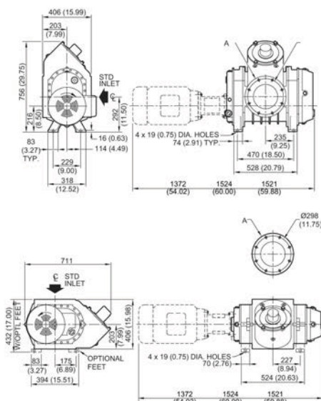
8" pipe flange connection 13 1/2" (343 mm) OD x 8" (203 mm) ID 8 x 3/4-10 NC-2B x 1 1/8" (29 mm) holes straddle both CL both flanges
