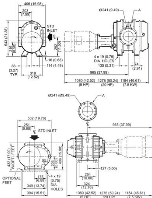
Standard dimensions: A - pipe flange connection 11" (279mm) OD x 6" (152mm) ID. 8 x 3/4-10 NC-2B x 1 1/8" (29mm) holes straddle both CL flanges
