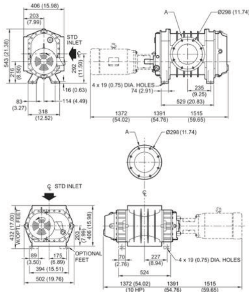
8" pipe flange connection 13 1/2" (343 mm) OD x 8" (203 mm) ID 8 x 3/4-10 NC-2B x 1 1/8" (29 mm) holes straddle both CL both flanges
