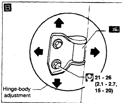
Door adjustment
