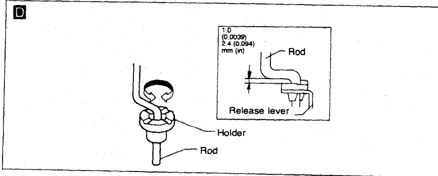
Outside handle adjustment
