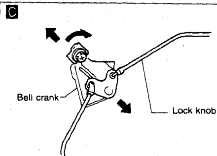
Bell crank adjustment
