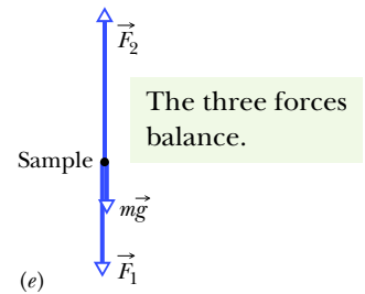
Figure 14.2.1 (a) A tank of water in which a sample of water is contained in an imaginary cylinder of horizontal base area A . (b)–(d) Force \vec{F}_1 acts at the top surface of the cylinder; force \vec{F}_2 acts at the bottom surface of the cylinder; the gravitational force on the water in the cylinder is represented by m\vec{g} . (e) A free-body diagram of the water sample. In WileyPLUS , this figure is available as an animation with voiceover.
