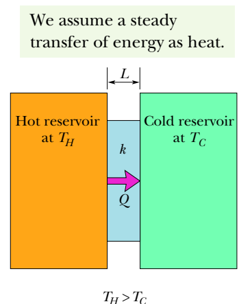
Figure 18.6.1 Thermal conduction. Energy is transferred as heat from a reservoir at temperature T_H to a cooler reservoir at temperature T_C through a conducting slab of thickness L and thermal conductivity k .
