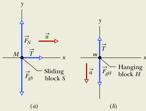
Figure 5.3.5 (a) A free-body diagram for block S of Fig. 5.3.3. (b) A free-body diagram for block H of Fig. 5.3.3.
