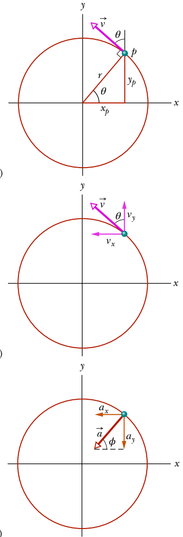
Figure 4.5.2 Particle p moves in counterclockwise uniform circular motion. (a) Its position and velocity \vec{v} at a certain instant. (b) Velocity \vec{v} . (c) Acceleration \vec{a} .
