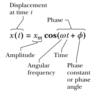
Figure 15.1.3 A handy guide to the quantities in Eq. 15.1.3 for simple harmonic motion.
