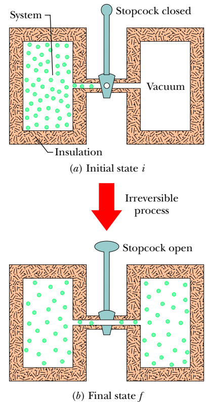
Figure 20.1.1 The free expansion of an ideal gas. (a) The gas is confined to the left half of an insulated container by a closed stopcock. (b) When the stopcock is opened, the gas rushes to fill the entire container. This process is irreversible; that is, it does not occur in reverse, with the gas spontaneously collecting itself in the left half of the container.
