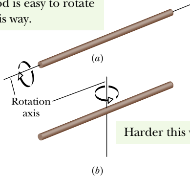
Figure 10.4.1 A long rod is much easier to rotate about (a) its central (longitudinal) axis than about (b) an axis through its center and perpendicular to its length. The reason for the difference is that the mass is distributed closer to the rotation axis in (a) than in (b).
