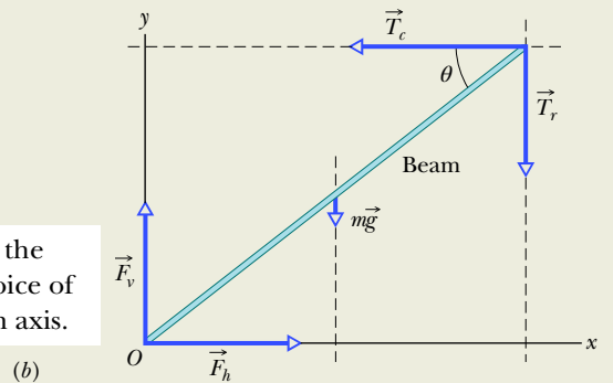
Figure 12.2.2 (a) A heavy safe is hung from a boom consisting of a horizontal steel cable and a uniform beam. (b) A free-body diagram for the beam.
