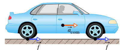
Figure 8.5.3 A vehicle accelerates to the right using four-wheel drive. The road exerts four frictional forces (two of them shown) on the bottom surfaces of the tires. Taken together, these four forces make up the net external force \vec{F} acting on the car.
