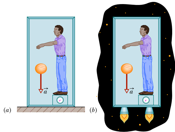
Figure 13.8.1 (a) A physicist in a box resting on Earth sees a cantaloupe falling with acceleration a = 9.8 \text{ m/s}^2 . (b) If he and the box accelerate in deep space at 9.8 \text{ m/s}^2 , the cantaloupe has the same acceleration relative to him. It is not possible, by doing experiments within the box, for the physicist to tell which situation he is in. For example, the platform scale on which he stands reads the same weight in both situations.
