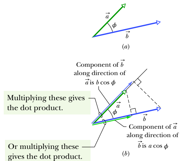
Figure 3.3.1 (a) Two vectors \vec{a} and \vec{b} , with an angle \phi between them. (b) Each vector has a component along the direction of the other vector.
