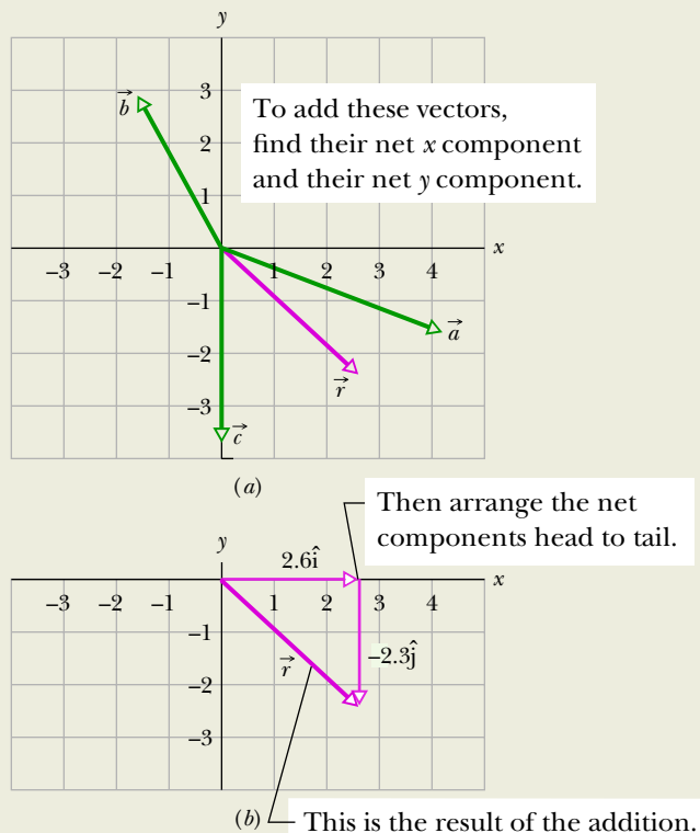
Figure 3.2.4 Vector \vec{r} is the vector sum of the other three vectors. where the minus sign means clockwise.
