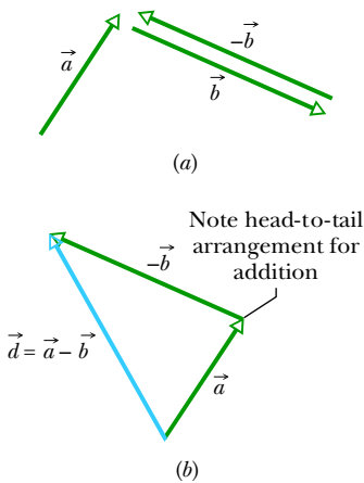
Figure 3.1.6 (a) Vectors \vec{a} , \vec{b} , and -\vec{b} . (b) To subtract vector \vec{b} from vector \vec{a} , add vector -\vec{b} to vector \vec{a} .
