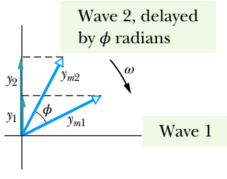
Figure 16.6.1 (a)–(d) A phasor of magnitude y_{m1} rotating about an origin at angular speed \omega represents a sinusoidal wave. The phasor's projection y_1 on the vertical axis represents the displacement of a point through which the wave passes. (e) A second phasor, also of angular speed \omega but of magnitude y_{m2} and rotating at a constant angle \phi from the first phasor, represents a second wave, with a phase constant \phi . (f) The resultant wave is represented by the vector sum y'_m of the two phasors.
