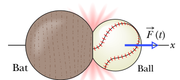
Figure 9.4.2 Force \vec{F}(t) acts on a ball as the ball and a bat collide.
