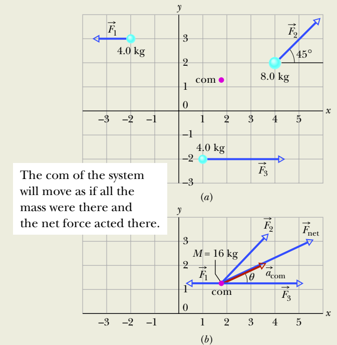
Figure 9.2.3 (a) Three particles, initially at rest in the positions shown, are acted on by the external forces shown. The center of mass (com) of the system is marked. (b) The forces are now transferred to the center of mass of the system, which behaves like a particle with a mass M equal to the total mass of the system. The net external force \vec{F}_{\text{net}} and the acceleration \vec{a}_{\text{com}} of the center of mass are shown.
