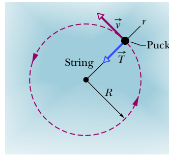
Figure 6.3.1 An overhead view of a hockey puck moving with constant speed v in a circular path of radius R on a horizontal frictionless surface. The centripetal force on the puck is \vec{T} , the pull from the string, directed inward along the radial axis r extending through the puck.
