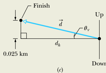
Figure 3.1.9 (a) Part of the Mammoth–Flint cave system, with the spelunking team’s route from Austin Entrance to Echo River indicated in red. (b) The components of the team’s overall displacement and their horizontal displacement d_h . (c) A side view showing d_h and the team’s overall displacement vector \vec{d} . (d) Team member Richard Zopf pushes his pack through the Tight Tube, near the bottom of the map. (Map adapted from map by The Cave Research Foundation. Photo courtesy of David des Marais, © The Cave Research Foundation)
