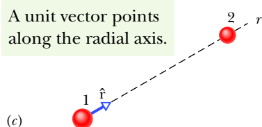
Figure 13.1.2 (a) The gravitational force \vec{F} on particle 1 due to particle 2 is an attractive force because particle 1 is attracted to particle 2. (b) Force \vec{F} is directed along a radial coordinate axis r extending from particle 1 through particle 2. (c) \vec{F} is in the direction of a unit vector \hat{r} along the r axis.
