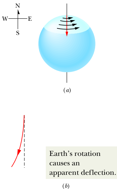
Figure 5.1.2 (a) The path of a puck sliding from the north pole as seen from a stationary point in space. Earth rotates to the east. (b) The path of the puck as seen from the ground.
