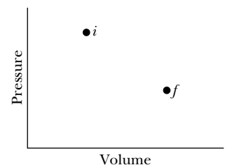
Figure 20.1.2 A p - V diagram showing the initial state i and the final state f of the free expansion of Fig. 20.1.1. The intermediate states of the gas cannot be shown because they are not equilibrium states.
