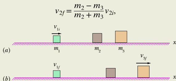
Figure 9.7.3 Block 1 collides with stationary block 2, which then collides with stationary block 3.
