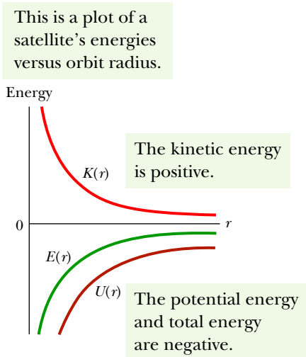
Figure 13.7.2 The variation of kinetic energy K , potential energy U , and total energy E with radius r for a satellite in a circular orbit. For any value of r , the values of U and E are negative, the value of K is positive, and E = -K . As r \rightarrow \infty , all three energy curves approach a value of zero.
