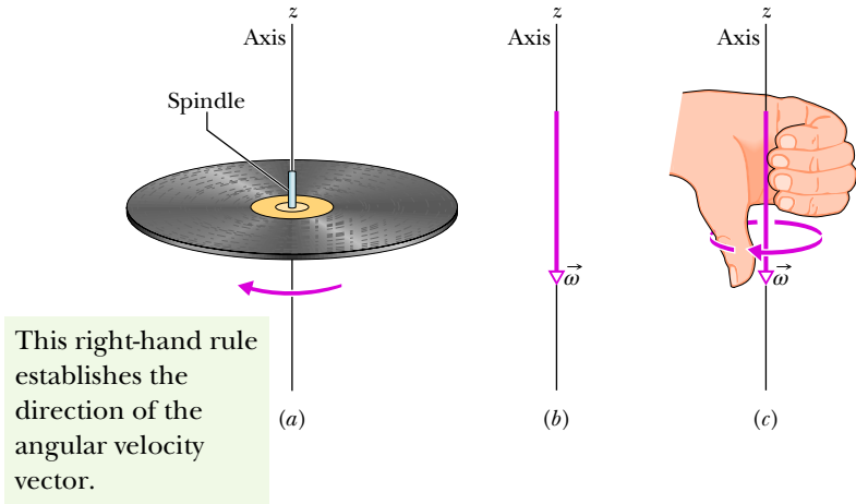
Figure 10.1.6 (a) A record rotating about a vertical axis that coincides with the axis of the spindle. (b) The angular velocity of the rotating record can be represented by the vector \vec{\omega} , lying along the axis and pointing down, as shown. (c) We establish the direction of the angular velocity vector as downward by using a right-hand rule. When the fingers of the right hand curl around the record and point the way it is moving, the extended thumb points in the direction of \vec{\omega} .
