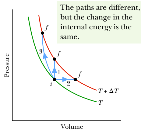
Figure 19.7.2 Three paths representing three different processes that take an ideal gas from an initial state i at temperature T to some final state f at temperature T + \Delta T . The change \Delta E_{\text{int}} in the internal energy of the gas is the same for these three processes and for any others that result in the same change of temperature.
