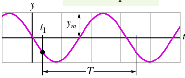
Figure 16.15 A graph of the displacement of the string element at x = 0 as a function of time, as the sinusoidal wave of Fig. 16.1.4 passes through the element. The amplitude y_m is indicated. A typical period T , measured from an arbitrary time t_1 , is also indicated.
