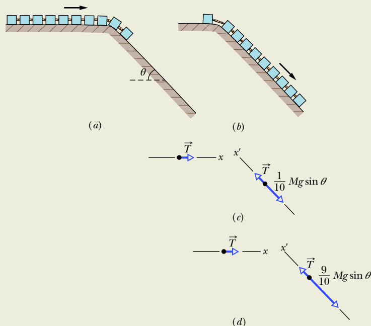
Figure 5.3.7 A roller coaster with (a) the first car on a slope and (b) all but the last car on the slope. (c) Free-body diagrams for the cars on the plateau and the car on the slope in (a). (d) Free-body diagrams for (b).
