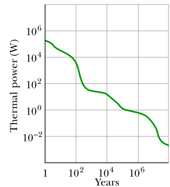
Figure 43.2.3 The thermal power released by the radioactive wastes from one year's operation of a typical large nuclear power plant, shown as a function of time. The curve is the superposition of the effects of many radionuclides, with a wide variety of half-lives. Note that both scales are logarithmic.
