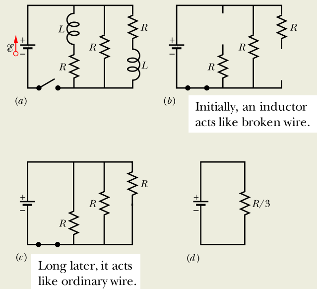
Figure 30.6.4 (a) A multiloop RL circuit with an open switch. (b) The equivalent circuit just after the switch has been closed. (c) The equivalent circuit a long time later. (d) The single-loop circuit that is equivalent to circuit (c).
