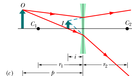
Figure 34.4.2 (a) A real, inverted image I is formed by a converging lens when the object O is outside the focal point F_1 . (b) The image I is virtual and has the same orientation as O when O is inside the focal point. (c) A diverging lens forms a virtual image I , with the same orientation as the object O , whether O is inside or outside the focal point of the lens.
