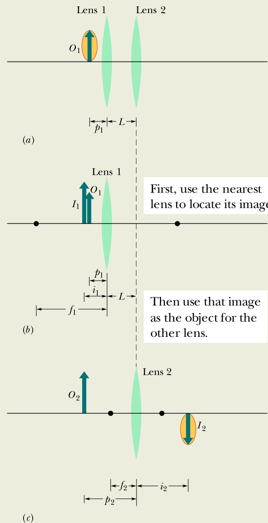
Figure 34.4.5 (a) Seed O_1 is distance p_1 from a two-lens system with lens separation L . We use the arrow to orient the seed. (b) The image I_1 produced by lens 1 alone. (c) Image I_1 acts as object O_2 for lens 2 alone, which produces the final image I_2 .
