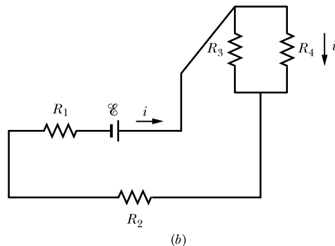
Figure 27.66 Problem 100. (a) An eel leaping up to a volunteer's arm in an experiment. (b) Circuit diagram for eel shocking the arm. (After Kenneth C. Catania, Department of Biological Sciences, Vanderbilt University)
