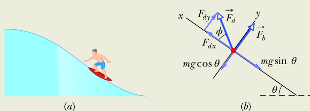
Figure 14.5.3 (a) Surfer. (b) Free-body diagram showing the forces on the surfer-surfboard system.
