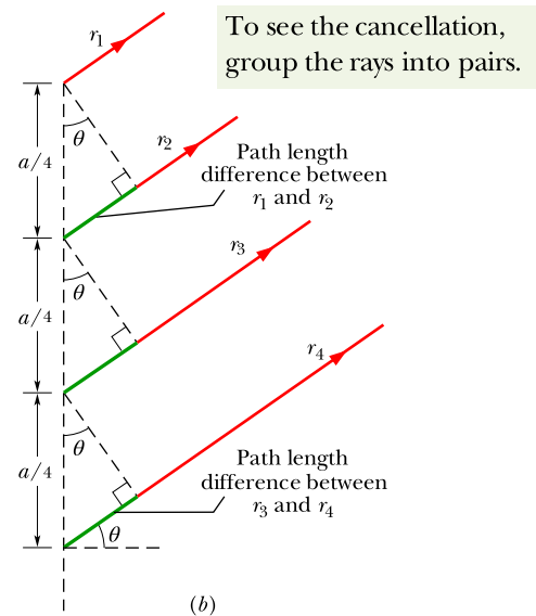
Figure 36.1.6 (a) Waves from the top points of four zones of width a/4 undergo fully destructive interference at point P_2 . (b) For D \gg a , we can approximate rays r_1, r_2, r_3, and r_4 as being parallel, at angle \theta to the central axis.
