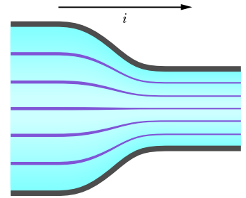
Figure 26.2.1 Streamlines representing current density in the flow of charge through a constricted conductor.
