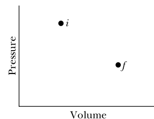
Figure 20.1.2 A p - V diagram showing the initial state i and the final state f of the free expansion of Fig. 20.1.1. The intermediate states of the gas cannot be shown because they are not equilibrium states.
