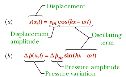
Figure 17.2.2 (a) The displacement function and (b) the pressure-variation function of a traveling sound wave consist of an amplitude and an oscillating term.
