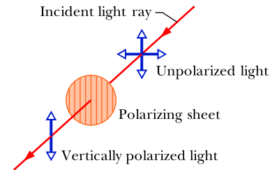
Figure 33.4.3 Unpolarized light becomes polarized when it is sent through a polarizing sheet. Its direction of polarization is then parallel to the polarizing direction of the sheet, which is represented here by the vertical lines drawn in the sheet.
