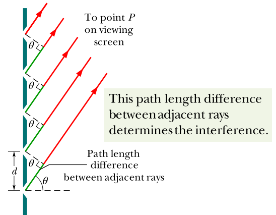
Figure 36.5.3 The rays from the rulings in a diffraction grating to a distant point P are approximately parallel. The path length difference between each two adjacent rays is d \sin \theta , where \theta is measured as shown. (The rulings extend into and out of the page.)
