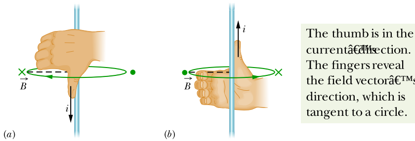
Figure 29.1.5 A right-hand rule gives the direction of the magnetic field due to a current in a wire. (a) The situation of Fig. 29.1.2, seen from the side. The magnetic field \vec{B} at any point to the left of the wire is perpendicular to the dashed radial line and directed into the page, in the direction of the fingertips, as indicated by the \otimes . (b) If the current is reversed, \vec{B} at any point to the left is still perpendicular to the dashed radial line but now is directed out of the page, as indicated by the \odot .
