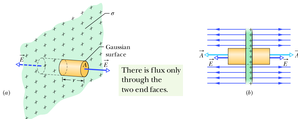
Figure 23.5.1 (a) Perspective view and (b) side view of a portion of a very large, thin plastic sheet, uniformly charged on one side to surface charge density \sigma . A closed cylindrical Gaussian surface passes through the sheet and is perpendicular to it.
