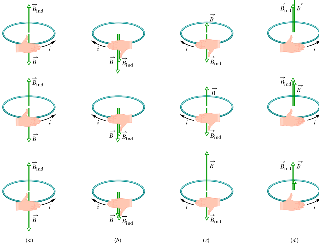
Figure 30.1.5 The direction of the current i induced in a loop is such that the current's magnetic field \vec{B}_{\text{ind}} opposes the change in the magnetic field \vec{B} inducing i . The field \vec{B}_{\text{ind}} is always directed opposite an increasing field \vec{B} (a, c) and in the same direction as a decreasing field \vec{B} (b, d). The curled-straight right-hand rule gives the direction of the induced current based on the direction of the induced field.
