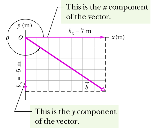
Figure 3.1.8 The component of \vec{b} on the x axis is positive, and that on the y axis is negative.
