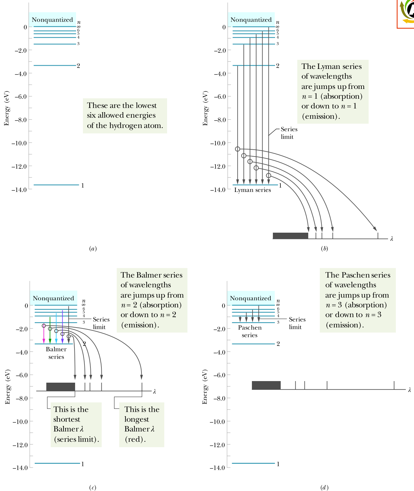
Figure 39.5.3 (a) An energy-level diagram for the hydrogen atom. Some of the transitions for (b) the Lyman series, (c) the Balmer series, and (d) the Paschen series. For each, the longest four wavelengths and the series-limit wavelength are plotted on a wavelength axis. Any wavelength shorter than the series-limit wavelength is allowed.
