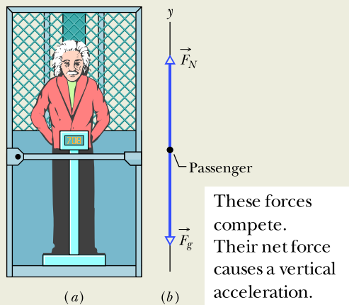
Figure 5.38 (a) A passenger stands on a platform scale that indicates either his weight or his apparent weight. (b) The free-body diagram for the passenger, showing the normal force \vec{F}_N on him from the scale and the gravitational force \vec{F}_g .
