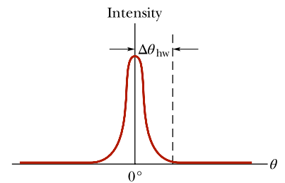
Figure 36.5.4 The half-width \Delta\theta_{\text{hw}} of the central line is measured from the center of that line to the adjacent minimum on a plot of I versus \theta like Fig. 36.5.2 a .
