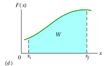
Figure 7.5.1 (a) A one-dimensional force \vec{F}(x) plotted against the displacement x of a particle on which it acts. The particle moves from x_i to x_f . (b) Same as (a) but with the area under the curve divided into narrow strips. (c) Same as (b) but with the area divided into narrower strips. (d) The limiting case. The work done by the force is given by Eq. 7.5.4 and is represented by the shaded area between the curve and the x axis and between x_i and x_f .
