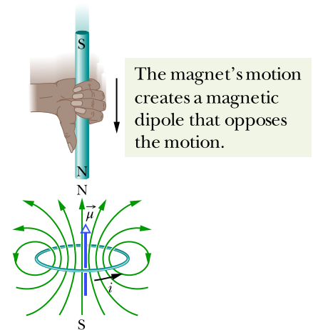
Figure 30.1.4 Lenz's law at work. As the magnet is moved toward the loop, a current is induced in the loop. The current produces its own magnetic field, with magnetic dipole moment \vec{\mu} oriented so as to oppose the motion of the magnet. Thus, the induced current must be counterclockwise as shown.
