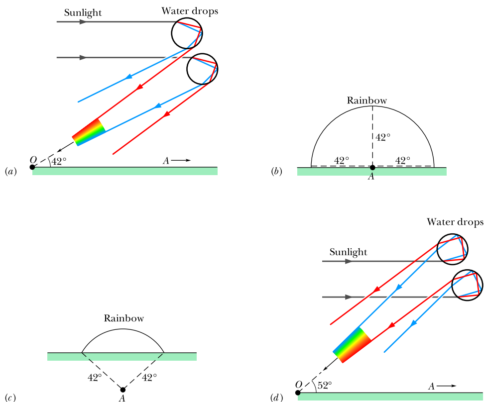
Figure 33.5.6 (a) The separation of colors when sunlight refracts into and out of falling raindrops leads to a primary rainbow. The antisolar point A is on the horizon at the right. The rainbow colors appear at an angle of 42^\circ from the direction of A . (b) Drops at 42^\circ from A in any direction can contribute to the rainbow. (c) The rainbow arc when the Sun is higher (and thus A is lower). (d) The separation of colors leading to a secondary rainbow.
