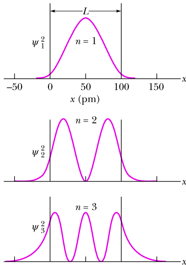
Figure 39.3.2 The first three probability densities \psi_n^2(x) for an electron confined to a finite potential well of depth U_0 = 450 eV and width L = 100 pm. Only states n = 1, 2, 3, and 4 are allowed.
