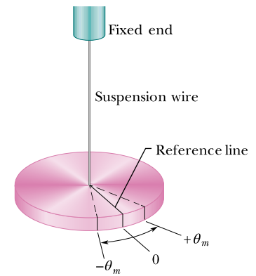
Figure 15.3.1 A torsion pendulum is an angular version of a linear simple harmonic oscillator. The disk oscillates in a horizontal plane; the reference line oscillates with angular amplitude \theta_m . The twist in the suspension wire stores potential energy as a spring does and provides the restoring torque.
