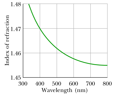
Figure 33.5.3 The index of refraction as a function of wavelength for fused quartz. The graph indicates that a beam of short-wavelength light, for which the index of refraction is higher, is bent more upon entering or leaving quartz than a beam of long-wavelength light.
