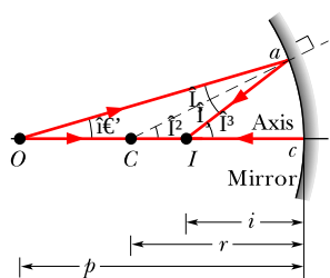
Figure 34.6.1 A concave spherical mirror forms a real point image I by reflecting light rays from a point object O .
