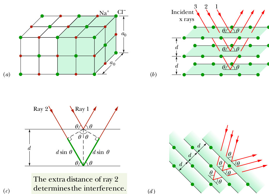
Figure 36.7.2 (a) The cubic structure of \text{NaCl} , showing the sodium and chlorine ions and a unit cell (shaded). (b) Incident x rays undergo diffraction by the structure of (a). The x rays are diffracted as if they were reflected by a family of parallel planes, with angles measured relative to the planes (not relative to a normal as in optics). (c) The path length difference between waves effectively reflected by two adjacent planes is 2d \sin \theta . (d) A different orientation of the incident x rays relative to the structure. A different family of parallel planes now effectively reflects the x rays.
