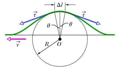
Figure 16.2.1 A symmetrical pulse, viewed from a reference frame in which the pulse is stationary and the string appears to move right to left with speed v . We find speed v by applying Newton's second law to a string element of length \Delta l , located at the top of the pulse.
