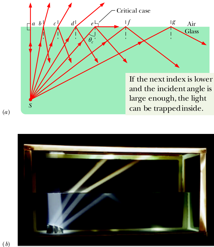
Figure 33.6.1 (a) Total internal reflection of light from a point source S in glass occurs for all angles of incidence greater than the critical angle \theta_c . At the critical angle, the refracted ray points along the air–glass interface. (b) A source in a tank of water.
