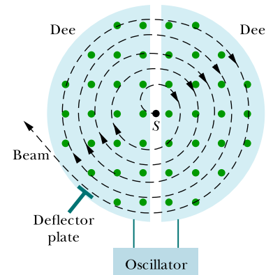
Figure 28.5.1 The elements of a cyclotron, showing the particle source S and the dees. A uniform magnetic field is directed up from the plane of the page. Circulating protons spiral outward within the hollow dees, gaining energy every time they cross the gap between the dees.
