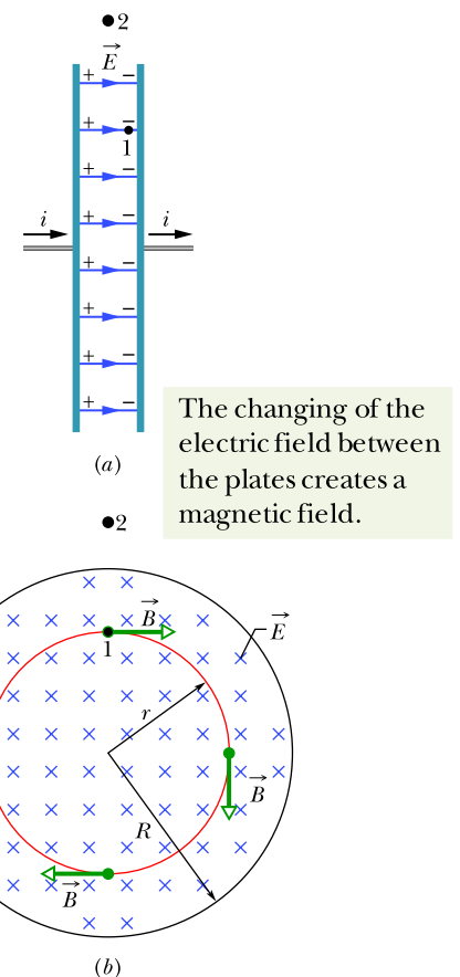
Figure 32.2.1 (a) A circular parallel-plate capacitor, shown in side view, is being charged by a constant current i . (b) A view from within the capacitor, looking toward the plate at the right in (a). The electric field \vec{E} is uniform, is directed into the page (toward the plate), and grows in magnitude as the charge on the capacitor increases. The magnetic field \vec{B} induced by this changing electric field is shown at four points on a circle with a radius r less than the plate radius R .
