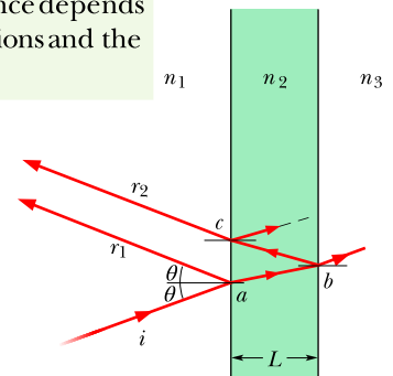
Figure 35.4.1 Light waves, represented with ray i , are incident on a thin film of thickness L and index of refraction n_2 . Rays r_1 and r_2 represent light waves that have been reflected by the front and back surfaces of the film, respectively. (All three rays are actually nearly perpendicular to the film.) The interference of the waves of r_1 and r_2 with each other depends on their phase difference. The index of refraction n_1 of the medium at the left can differ from the index of refraction n_3 of the medium at the right, but for now we assume that both media are air, with n_1 = n_3 = 1.0 , which is less than n_2 .
