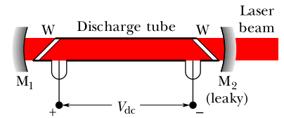
Figure 40.7.4 The elements of a helium–neon gas laser. An applied potential V_{dc} sends electrons through a discharge tube containing a mixture of helium gas and neon gas. Electrons collide with helium atoms, which then collide with neon atoms, which emit light along the length of the tube. The light passes through transparent windows W and reflects back and forth through the tube from mirrors M_1 and M_2 to cause more neon atom emissions. Some of the light leaks through mirror M_2 to form the laser beam.
