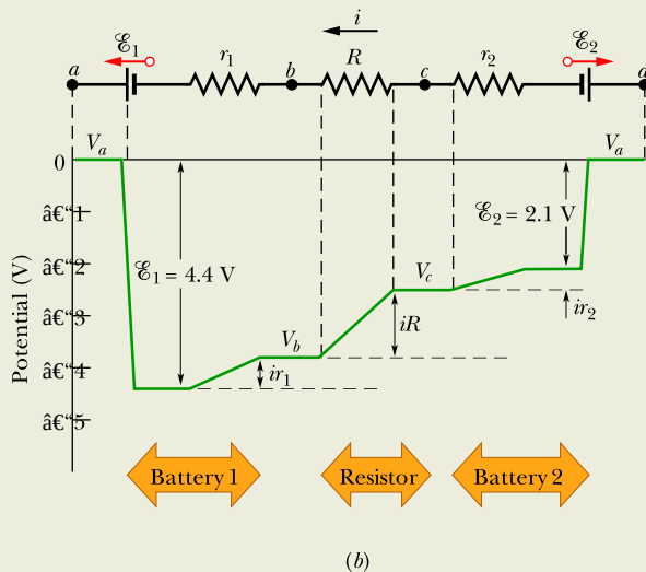
Figure 27.1.8 (a) A single-loop circuit containing two real batteries and a resistor. The batteries oppose each other; that is, they tend to send current in opposite directions through the resistor. (b) A graph of the potentials, counterclockwise from point a , with the potential at a arbitrarily taken to be zero. (To better link the circuit with the graph, mentally cut the circuit at a and then unfold the left side of the circuit toward the left and the right side of the circuit toward the right.)
