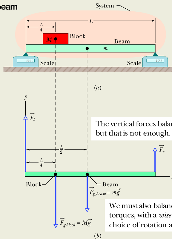
Figure 12.2.1 (a) A beam of mass m supports a block of mass M . (b) A free-body diagram, showing the forces that act on the system beam + block .
