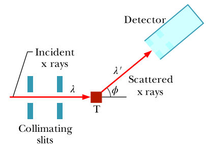
Figure 38.3.1 Compton's apparatus. A beam of x rays of wavelength \lambda = 71.1 pm is directed onto a carbon target T. The x rays scattered from the target are observed at various angles \phi to the direction of the incident beam. The detector measures both the intensity of the scattered x rays and their wavelength.
