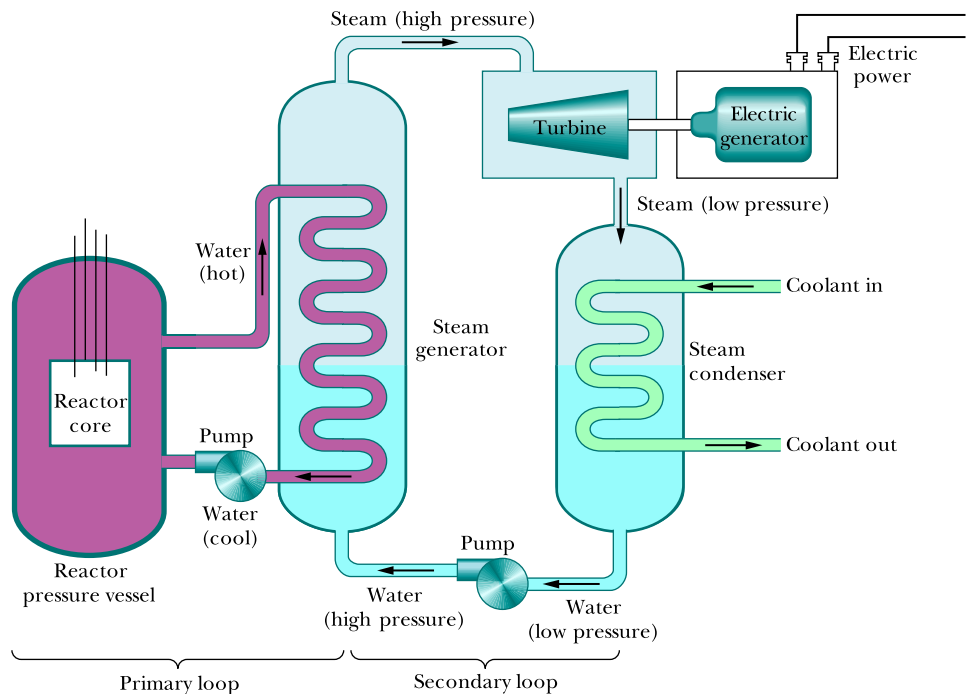
Figure 43.2.2 A simplified layout of a nuclear power plant, based on a pressurized-water reactor. Many features are omitted—among them the arrangement for cooling the reactor core in case of an emergency.
