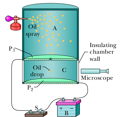
Figure 22.6.1 The Millikan oil-drop apparatus for measuring the elementary charge e . When a charged oil drop drifted into chamber C through the hole in plate P_1 , its motion could be controlled by closing and opening switch S and thereby setting up or eliminating an electric field in chamber C. The microscope was used to view the drop, to permit timing of its motion.
