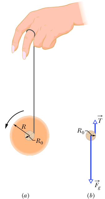
Figure 11.3.1 (a) A yo-yo, shown in cross section. The string, of assumed negligible thickness, is wound around an axle of radius R_0 . (b) A free-body diagram for the falling yo-yo. Only the axle is shown.
