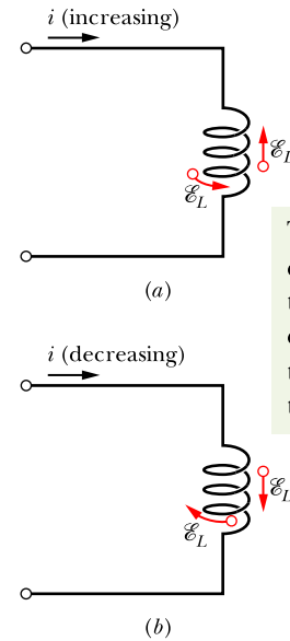
Figure 30.5.2 (a) The current i is increasing, and the self-induced emf \mathcal{E}_L appears along the coil in a direction such that it opposes the increase. The arrow representing \mathcal{E}_L can be drawn along a turn of the coil or alongside the coil. Both are shown. (b) The current i is decreasing, and the self-induced emf appears in a direction such that it opposes the decrease.
