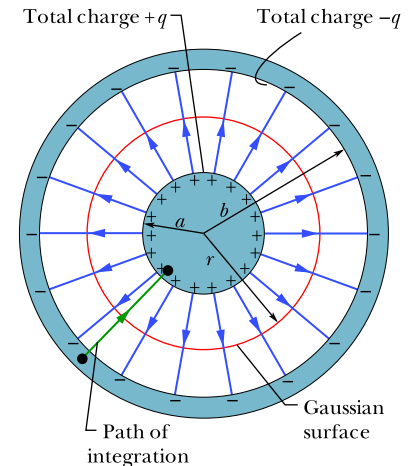
Figure 25.2.2 A cross section of a long cylindrical capacitor, showing a cylindrical Gaussian surface of radius r (that encloses the positive plate) and the radial path of integration along which Eq. 25.2.4 is to be applied. This figure also serves to illustrate a spherical capacitor in a cross section through its center.
