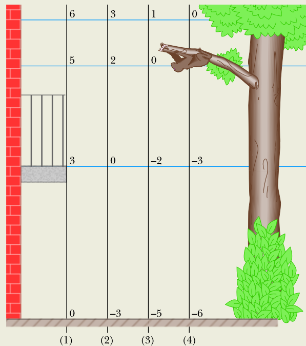
Figure 8.1.6 Four choices of reference point y = 0 . Each y axis is marked in units of meters. The choice affects the value of the potential energy U of the sloth–Earth system. However, it does not affect the change \Delta U in potential energy of the system if the sloth moves by, say, falling.
