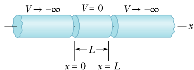
Figure 39.1.1 The elements of an idealized “trap” designed to confine an electron to the central cylinder. We take the semi-ininitely long end cylinders to be at an infinitely great negative potential and the central cylinder to be at zero potential.
