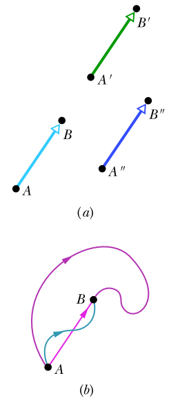
Figure 3.1.1 (a) All three arrows have the same magnitude and direction and thus represent the same displacement. (b) All three paths connecting the two points correspond to the same displacement vector.
