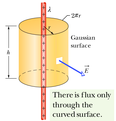
Figure 23.4.1 A Gaussian surface in the form of a closed cylinder surrounds a section of a very long, uniformly charged, cylindrical plastic rod.
