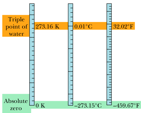
Figure 18.2.1 The Kelvin, Celsius, and Fahrenheit temperature scales compared.
