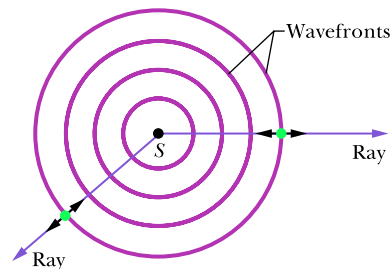
Figure 17.1.2 A sound wave travels from a point source S through a three-dimensional medium. The wavefronts form spheres centered on S ; the rays are radial to S . The short, double-headed arrows indicate that elements of the medium oscillate parallel to the rays.
