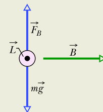
Figure 28.6.4 A wire (shown in cross section) carrying current out of the page.
