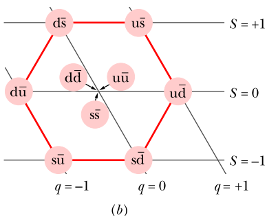
Figure 44.3.2 (a) The quark compositions of the eight spin- \frac{1}{2} baryons plotted in Fig. 44.2.1a. (Although the two central baryons share the same quark structure, they are different particles. The sigma is an excited state of the lambda, decaying into the lambda by emission of a gamma-ray photon.) (b) The quark compositions of the nine spin-zero mesons plotted in Fig. 44.2.1b.
