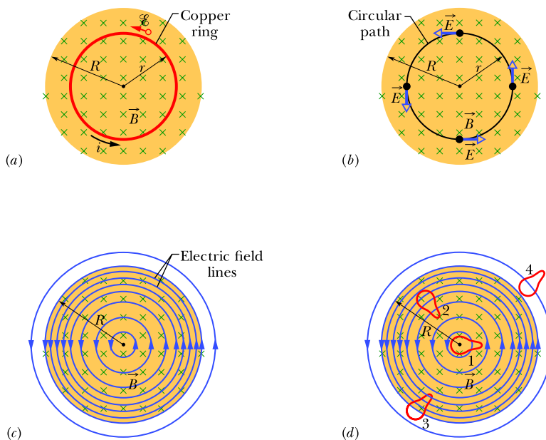
Figure 30.3.1 (a) If the magnetic field increases at a steady rate, a constant induced current appears, as shown, in the copper ring of radius r . (b) An induced electric field exists even when the ring is removed; the electric field is shown at four points. (c) The complete picture of the induced electric field, displayed as field lines. (d) Four similar closed paths that enclose identical areas. Equal emfs are induced around paths 1 and 2, which lie entirely within the region of changing magnetic field. A smaller emf is induced around path 3, which only partially lies in that region. No net emf is induced around path 4, which lies entirely outside the magnetic field.
