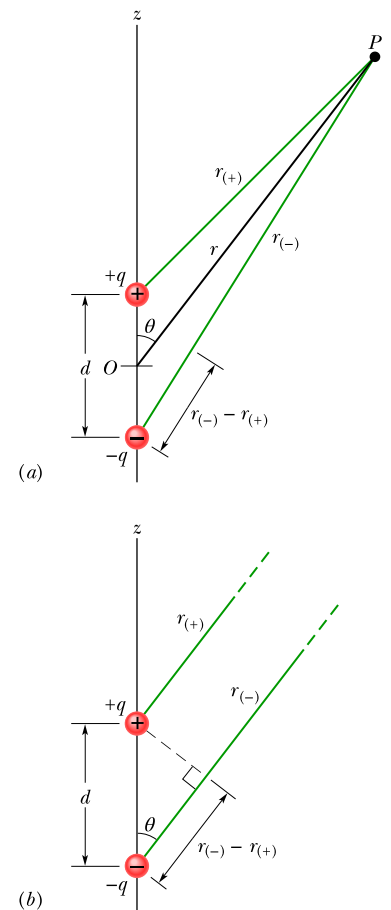
Figure 24.4.1 (a) Point P is a distance r from the midpoint O of a dipole. The line OP makes an angle \theta with the dipole axis. (b) If P is far from the dipole, the lines of lengths r_{(+)} and r_{(-)} are approximately parallel to the line of length r , and the dashed black line is approximately perpendicular to the line of length r_{(-)} .
