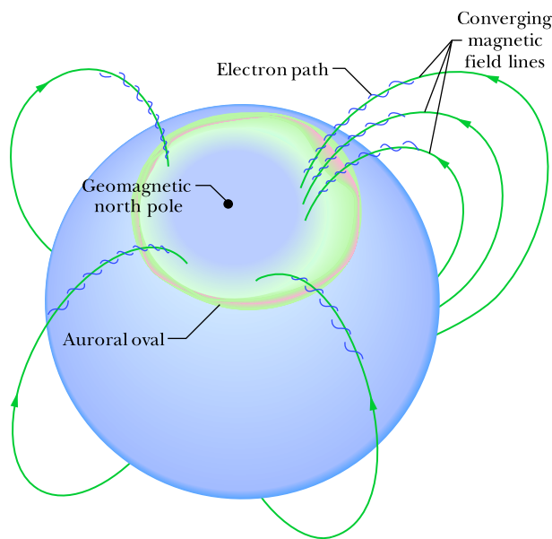
Figure 28.4.4 The auroral oval surrounding Earth's geomagnetic north pole (which is currently located near northwestern Greenland). Magnetic field lines converge toward that pole. Electrons moving toward Earth are "caught by" and spiral around these lines, entering the atmosphere at middle to high latitudes and producing auroras within the oval.
