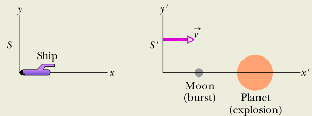
Figure 37.3.2 A planet and its moon in reference frame S' move rightward with speed v relative to a starship in reference frame S .
