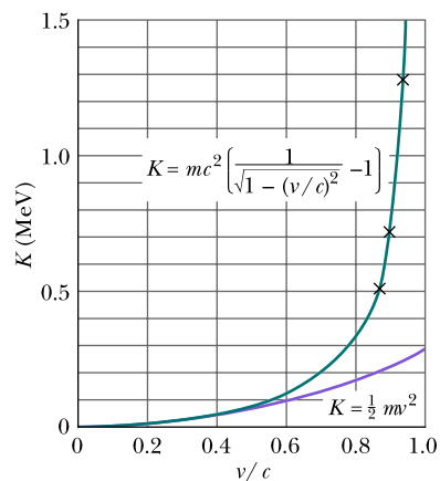
Figure 37.6.1 The relativistic (Eq. 37.6.13) and classical (Eq. 37.6.12) equations for the kinetic energy of an electron, plotted as a function of v/c , where v is the speed of the electron and c is the speed of light. Note that the two curves blend together at low speeds and diverge widely at high speeds. Experimental data (at the \times marks) show that at high speeds the relativistic curve agrees with experiment but the classical curve does not.
