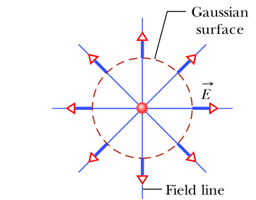
Figure 23.1.1 Electric field vectors and field lines pierce an imaginary, spherical Gaussian surface that encloses a particle with charge +Q .
