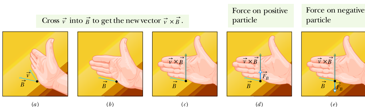
Figure 28.1.2 (a)–(c) The right-hand rule (in which \vec{v} is swept into \vec{B} through the smaller angle \phi between them) gives the direction of \vec{v} \times \vec{B} as the direction of the thumb. (d) If q is positive, then the direction of \vec{F}_B = q\vec{v} \times \vec{B} is in the direction of \vec{v} \times \vec{B} . (e) If q is negative, then the direction of \vec{F}_B is opposite that of \vec{v} \times \vec{B} .
