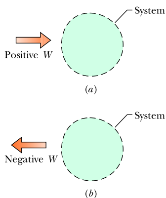
Figure 8.4.1 (a) Positive work W done on an arbitrary system means a transfer of energy to the system. (b) Negative work W means a transfer of energy from the system.
