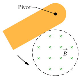
Figure 30.2.5 (a) As you pull a solid conducting plate out of a magnetic field, eddy currents are induced in the plate. A typical loop of eddy current is shown. (b) A conducting plate is allowed to swing like a pendulum about a pivot and into a region of magnetic field. As it enters and leaves the field, eddy currents are induced in the plate.
