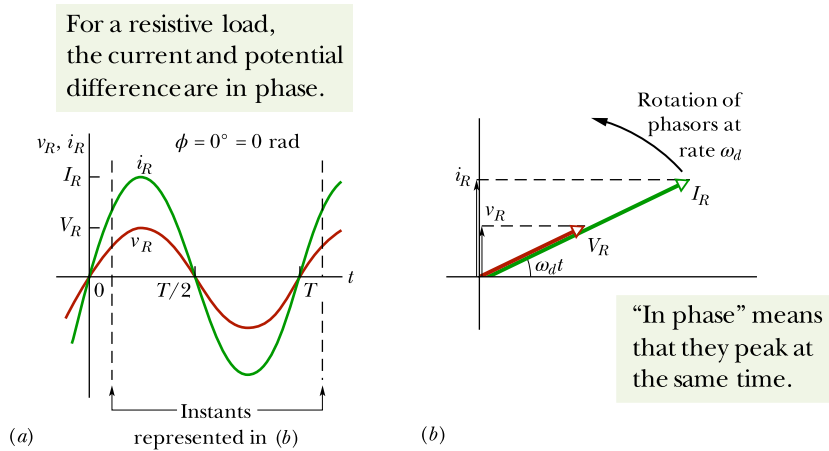
Figure 31.3.4 (a) The current i_R and the potential difference v_R across the resistor are plotted on the same graph, both versus time t . They are in phase and complete one cycle in one period T . (b) A phasor diagram shows the same thing as (a).
