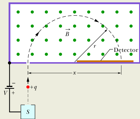
Figure 28.4.5 A positive ion is accelerated from its source S by a potential difference V , enters a chamber of uniform magnetic field \vec{B} , travels through a semicircle of radius r , and strikes a detector at a distance x .
