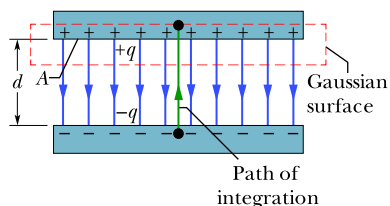
Figure 25.2.1 A charged parallel-plate capacitor. A Gaussian surface encloses the charge on the positive plate. The integration of Eq. 25.2.4 is taken along a path extending directly from the negative plate to the positive plate.
