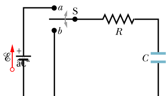
Figure 27.4.1 When switch S is closed on a , the capacitor is charged through the resistor. When the switch is afterward closed on b , the capacitor discharges through the resistor.
