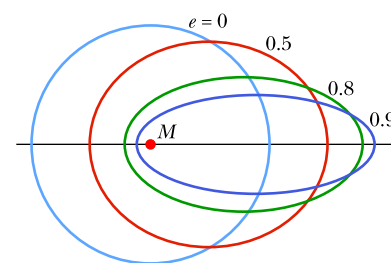
Figure 13.7.1 Four orbits with different eccentricities e about an object of mass M . All four orbits have the same semimajor axis a and thus correspond to the same total mechanical energy E .
