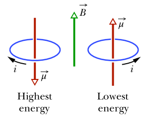
Figure 28.8.1 The orientations of highest and lowest energy of a magnetic dipole (here a coil carrying current) in an external magnetic field \vec{B} . The direction of the current i gives the direction of the magnetic dipole moment \vec{\mu} via the right-hand rule shown for \vec{n} in Fig. 28.7.2b.
