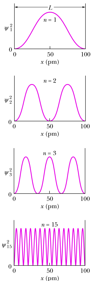
Figure 39.2.1 The probability density \psi_n^2(x) for four states of an electron trapped in a one-dimensional infinite well; their quantum numbers are n = 1, 2, 3 , and 15. The electron is most likely to be found where \psi_n^2(x) is greatest and least likely to be found where \psi_n^2(x) is least.
