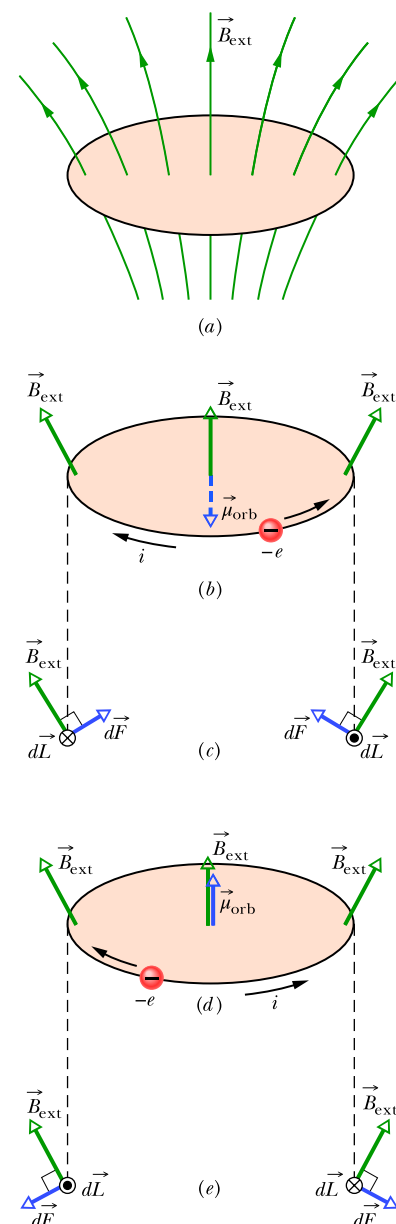
Figure 32.5.3 (a) A loop model for an electron orbiting in an atom while in a nonuniform magnetic field \vec{B}_{\text{ext}} . (b) Charge -e moves counterclockwise; the associated conventional current i is clockwise. (c) The magnetic forces d\vec{F} on the left and right sides of the loop, as seen from the plane of the loop. The net force on the loop is upward. (d) Charge -e now moves clockwise. (e) The net force on the loop is now downward.
