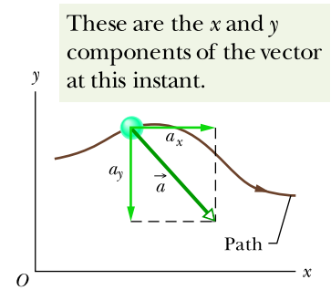
Figure 4.3.1 The acceleration \vec{a} of a particle and the scalar components of \vec{a} .
