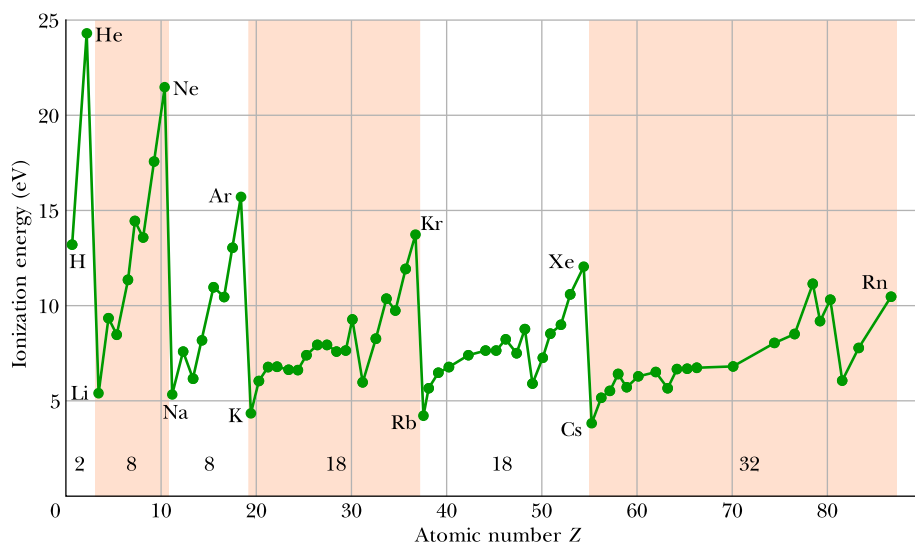
Figure 40.1.2 A plot of the ionization energies of the elements as a function of atomic number, showing the periodic repetition of properties through the six complete horizontal periods of the periodic table. The number of elements in each of these periods is indicated.
