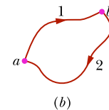
Figure 8.1.4 (a) As a conservative force acts on it, a particle can move from point a to point b along either path 1 or path 2. (b) The particle moves in a round trip, from point a to point b along path 1 and then back to point a along path 2.
