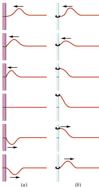
Figure 16.7.3 (a) A pulse incident from the right is reflected at the left end of the string, which is tied to a wall. Note that the reflected pulse is inverted from the incident pulse. (b) Here the left end of the string is tied to a ring that can slide without friction up and down the rod. Now the pulse is not inverted by the reflection.
