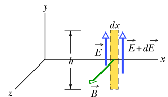
Figure 33.1.6 As the electromagnetic wave travels rightward past point P in Fig. 33.1.5b, the sinusoidal variation of the magnetic field \vec{B} through a rectangle centered at P induces electric fields along the rectangle. At the instant shown, \vec{B} is decreasing in magnitude and the induced electric field is therefore greater in magnitude on the right side of the rectangle than on the left.
