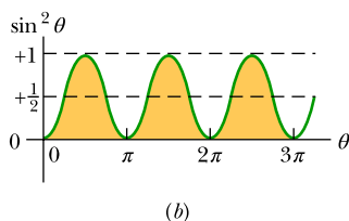
Figure 31.5.1 (a) A plot of \sin \theta versus \theta . The average value over one cycle is zero. (b) A plot of \sin^2 \theta versus \theta . The average value over one cycle is \frac{1}{2} .
