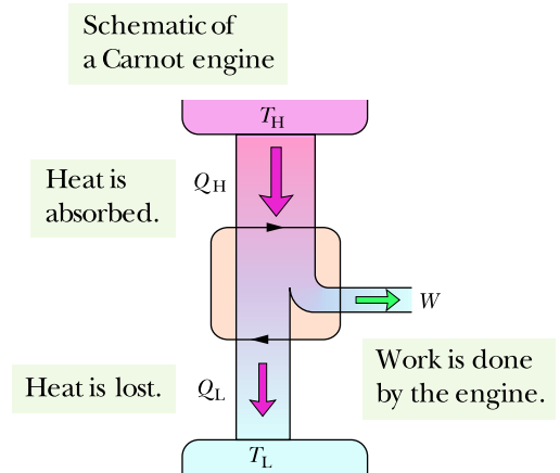
Figure 20.2.1 The elements of a Carnot engine. The two black arrowheads on the central loop suggest the working substance operating in a cycle, as if on a p - V plot. Energy |Q_H| is transferred as heat from the high-temperature reservoir at temperature T_H to the working substance. Energy |Q_L| is transferred as heat from the working substance to the low-temperature reservoir at temperature T_L . Work W is done by the engine (actually by the working substance) on something in the environment.
