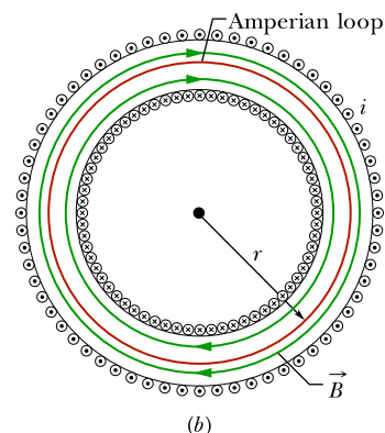
Figure 29.4.5 (a) A toroid carrying a current i . (b) A horizontal cross section of the toroid. The interior magnetic field (inside the bracelet-shaped tube) can be found by applying Ampere's law with the Amperian loop shown.
