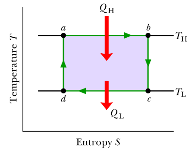
Figure 20.2.3 The Carnot cycle of Fig. 20.2.2 plotted on a temperature–entropy diagram. During processes ab and cd the temperature remains constant. During processes bc and da the entropy remains constant.
