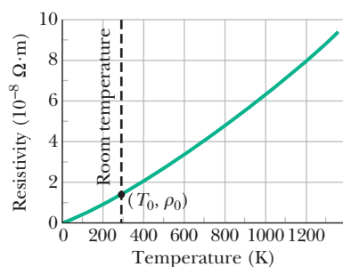
Figure 26-10 The resistivity of copper as a function of temperature. The dot on the curve marks a convenient reference point at temperature T_0 = 293 K and resistivity \rho_0 = 1.69 \times 10^{-8} \Omega \cdot \text{m} .
