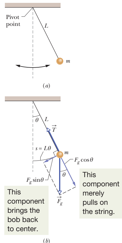
Figure 15-11 (a) A simple pendulum. (b) The forces acting on the bob are the gravitational force \vec{F}_g and the force \vec{T} from the string. The tangential component F_g \sin \theta of the gravitational force is a restoring force that tends to bring the pendulum back to its central position.
