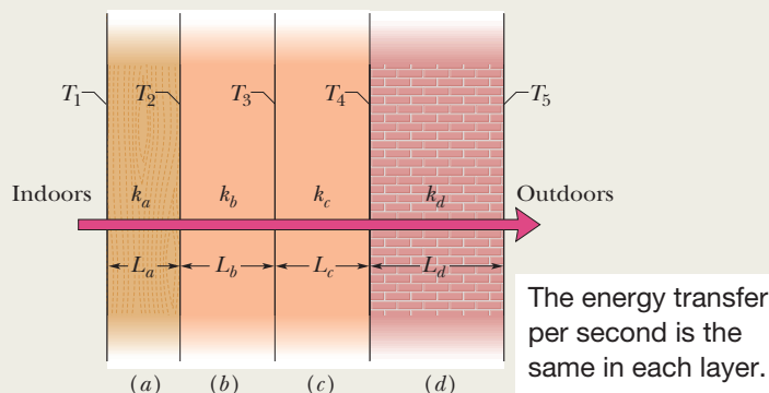
Figure 18-22 Steady-state heat transfer through a wall.
