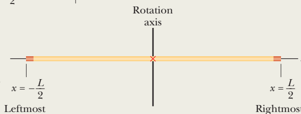
Figure 10-14 A uniform rod of length L and mass M . An element of mass dm and length dx is represented.
