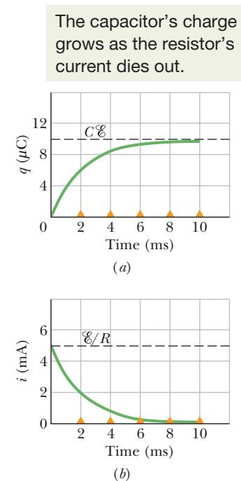
Figure 27-16 (a) A plot of Eq. 27-33, which shows the buildup of charge on the capacitor of Fig. 27-15. (b) A plot of Eq. 27-34, which shows the decline of the charging current in the circuit of Fig. 27-15. The curves are plotted for R = 2000 \Omega , C = 1 \mu\text{F} , and \mathcal{E} = 10 \text{ V} ; the small triangles represent successive intervals of one time constant \tau .
