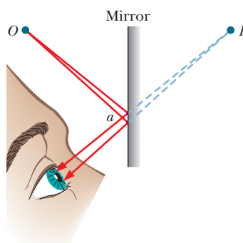
Figure 34-4 A “pencil” of rays from O enters the eye after reflection at the mirror. Only a small portion of the mirror near a is involved in this reflection. The light appears to originate at point I behind the mirror.
