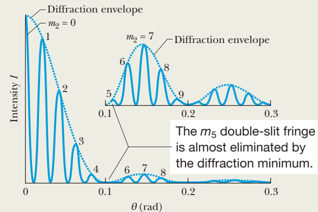
Figure 36-17 One side of the intensity plot for a two-slit interference experiment. The inset shows (vertically expanded) the plot within the first and second side peaks of the diffraction envelope.
