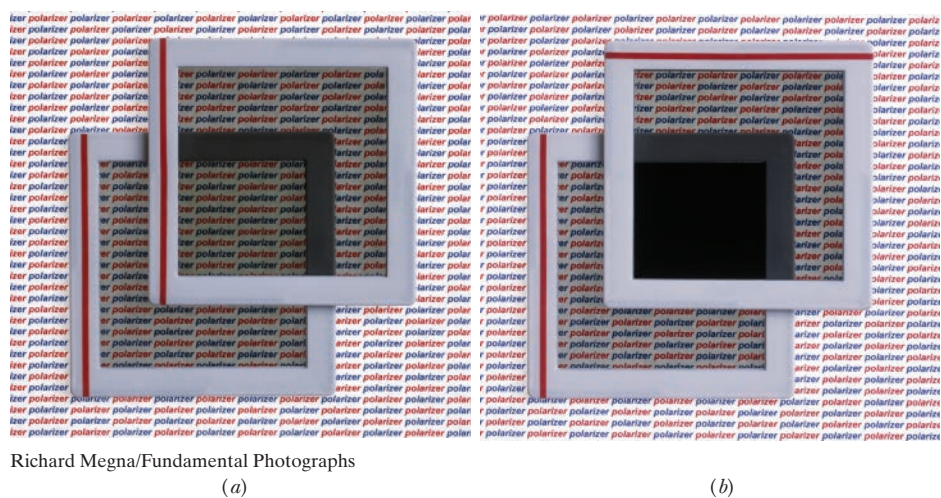
Figure 33-14 (a) Overlapping polarizing sheets transmit light fairly well when their polarizing directions have the same orientation, but (b) they block most of the light when they are crossed.
