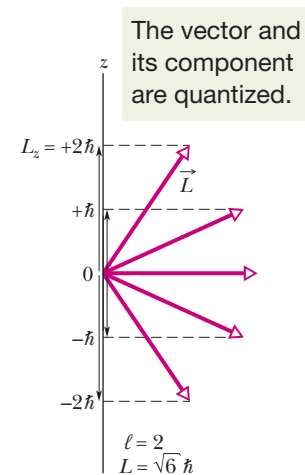
Figure 40-5 The allowed values of L_z for an electron in a quantum state with \ell = 2 . For every orbital angular momentum vector \vec{L} in the figure, there is a vector pointing in the opposite direction, representing the magnitude and direction of the orbital magnetic dipole moment \vec{\mu}_{\text{orb}} .
