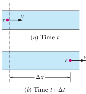
Figure 14-16 Fluid flows at a constant speed v through a tube. (a) At time t , fluid element e is about to pass the dashed line. (b) At time t + \Delta t , element e is a distance \Delta x = v \Delta t from the dashed line.
