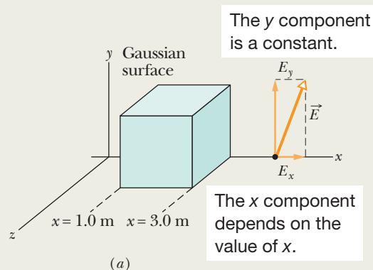
Figure 23-7 (a) A Gaussian cube with one edge on the x axis lies within a nonuniform electric field that depends on the value of x . (b) Each patch element has an outward vector that is perpendicular to the area. (c) Right face: the x component of the field pierces the area and produces positive (outward) flux. The y component does not pierce the area and thus does not produce any flux. (Figure continues on following page)
