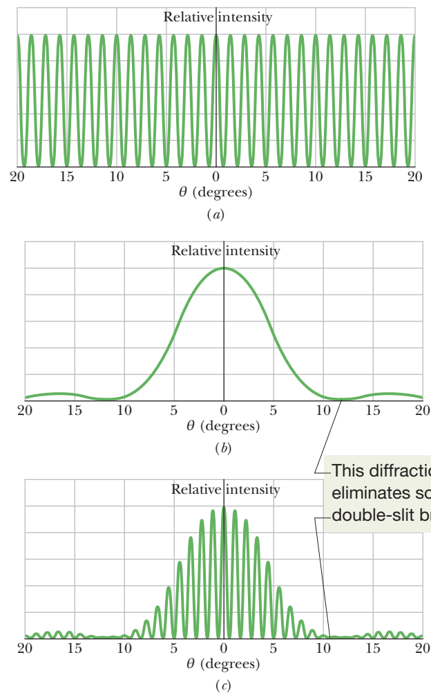
Figure 36-15 (a) The intensity plot to be expected in a double-slit interference experiment with vanishingly narrow slits. (b) The intensity plot for diffraction by a typical slit of width a (not vanishingly narrow). (c) The intensity plot to be expected for two slits of width a . The curve of (b) acts as an envelope, limiting the intensity of the double-slit fringes in (a). Note that the first minima of the diffraction pattern of (b) eliminate the double-slit fringes that would occur near 12^\circ in (c).
