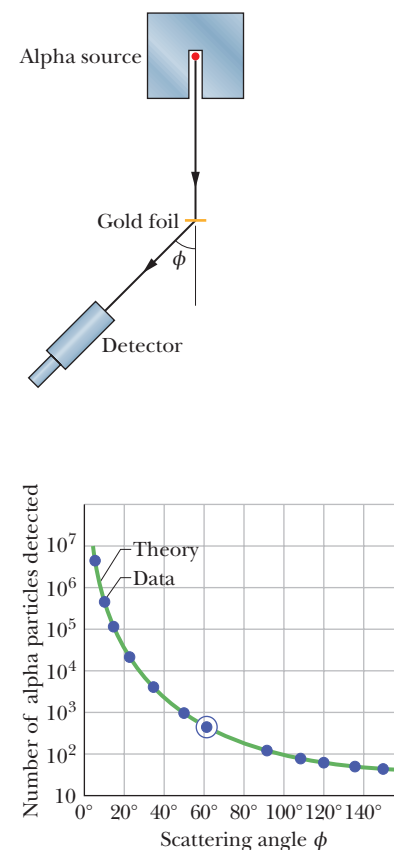
Figure 42-2 The dots are alpha-particle scattering data for a gold foil, obtained by Geiger and Marsden using the apparatus of Fig. 42-1. The solid curve is the theoretical prediction, based on the assumption that the atom has a small, massive, positively charged nucleus. The data have been adjusted to fit the theoretical curve at the experimental point that is enclosed in a circle.
