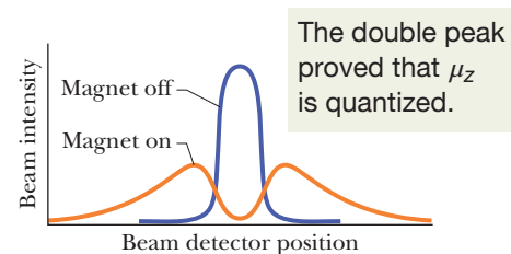
Figure 40-9 Results of a modern repetition of the Stern–Gerlach experiment. With the electromagnet turned off, there is only a single beam; with the electromagnet turned on, the original beam splits into two subbeams. The two subbeams correspond to parallel and antiparallel alignment of the magnetic moments of cesium atoms with the external magnetic field.
