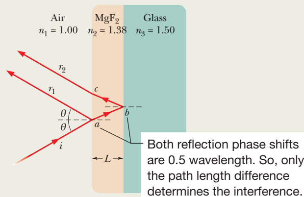
Figure 35-19 Unwanted reflections from glass can be suppressed (at a chosen wavelength) by coating the glass with a thin transparent film of magnesium fluoride of the properly chosen thickness.
