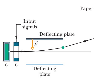
Figure 22-17 Ink-jet printer. Drops shot from generator G receive a charge in charging unit C . An input signal from a computer controls the charge and thus the effect of field \vec{E} on where the drop lands on the paper.
