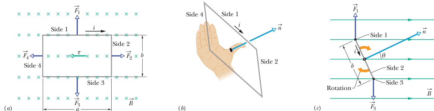
Figure 28-19 A rectangular loop, of length a and width b and carrying a current i , is located in a uniform magnetic field. A torque \tau acts to align the normal vector \vec{n} with the direction of the field. (a) The loop as seen by looking in the direction of the magnetic field. (b) A perspective of the loop showing how the right-hand rule gives the direction of \vec{n} , which is perpendicular to the plane of the loop. (c) A side view of the loop, from side 2. The loop rotates as indicated.
