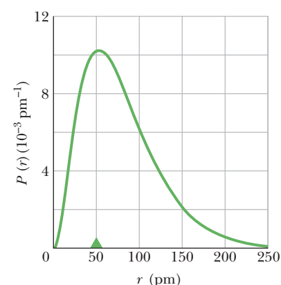
Figure 39-19 A plot of the radial probability density P(r) for the ground state of the hydrogen atom. The triangular marker is located at one Bohr radius from the origin, and the origin represents the center of the atom.
