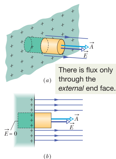
Figure 23-12 (a) Perspective view and (b) side view of a tiny portion of a large, isolated conductor with excess positive charge on its surface. A (closed) cylindrical Gaussian surface, embedded perpendicularly in the conductor, encloses some of the charge. Electric field lines pierce the external end cap of the cylinder, but not the internal end cap. The external end cap has area A and area vector \vec{A} .
