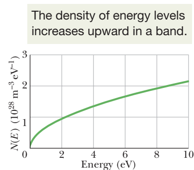
Figure 41-6 The density of states N(E) — that is, the number of electron energy levels per unit energy interval per unit volume — plotted as a function of electron energy. The density of states function simply counts the available states; it says nothing about whether these states are occupied by electrons.
