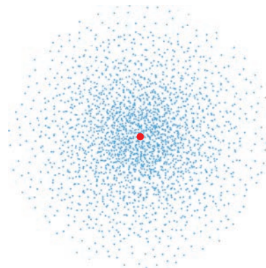
Figure 39-20 A “dot plot” showing the volume probability density \psi^2(r) — not the radial probability density P(r) — for the ground state of the hydrogen atom. The density of dots drops exponentially with increasing distance from the nucleus, which is represented here by a red spot.
