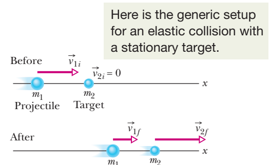
Figure 9-18 Body 1 moves along an x axis before having an elastic collision with body 2, which is initially at rest. Both bodies move along that axis after the collision.
