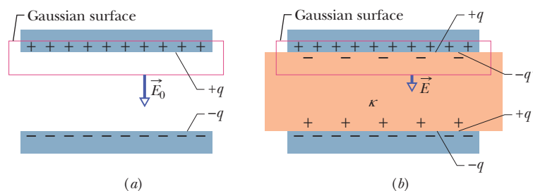
Figure 25-16 A parallel-plate capacitor (a) without and (b) with a dielectric slab inserted. The charge q on the plates is assumed to be the same in both cases.
