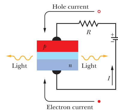
Figure 41-16 A forward-biased p - n junction, showing electrons being injected into the n -type material and holes into the p -type material. (Holes move in the conventional direction of the current I , equivalent to electrons moving in the opposite direction.) Light is emitted from the narrow depletion zone each time an electron and a hole combine across that zone.
