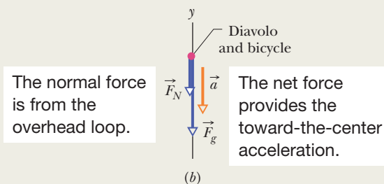
Figure 6-9 (a) Contemporary advertisement for Diavolo and (b) free-body diagram for the performer at the top of the loop.
