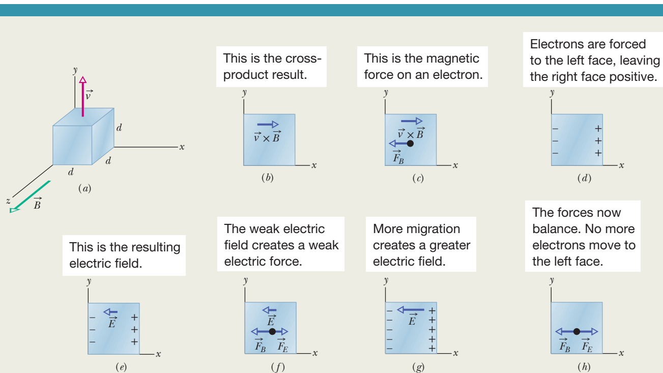
Figure 28-9 (a) A solid metal cube moves at constant velocity through a uniform magnetic field. (b)–(d) In these front views, the magnetic force acting on an electron forces the electron to the left face, making that face negative and leaving the opposite face positive. (e)–(f) The resulting weak electric field creates a weak electric force on the next electron, but it too is forced to the left face. Now (g) the electric field is stronger and (h) the electric force matches the magnetic force.
