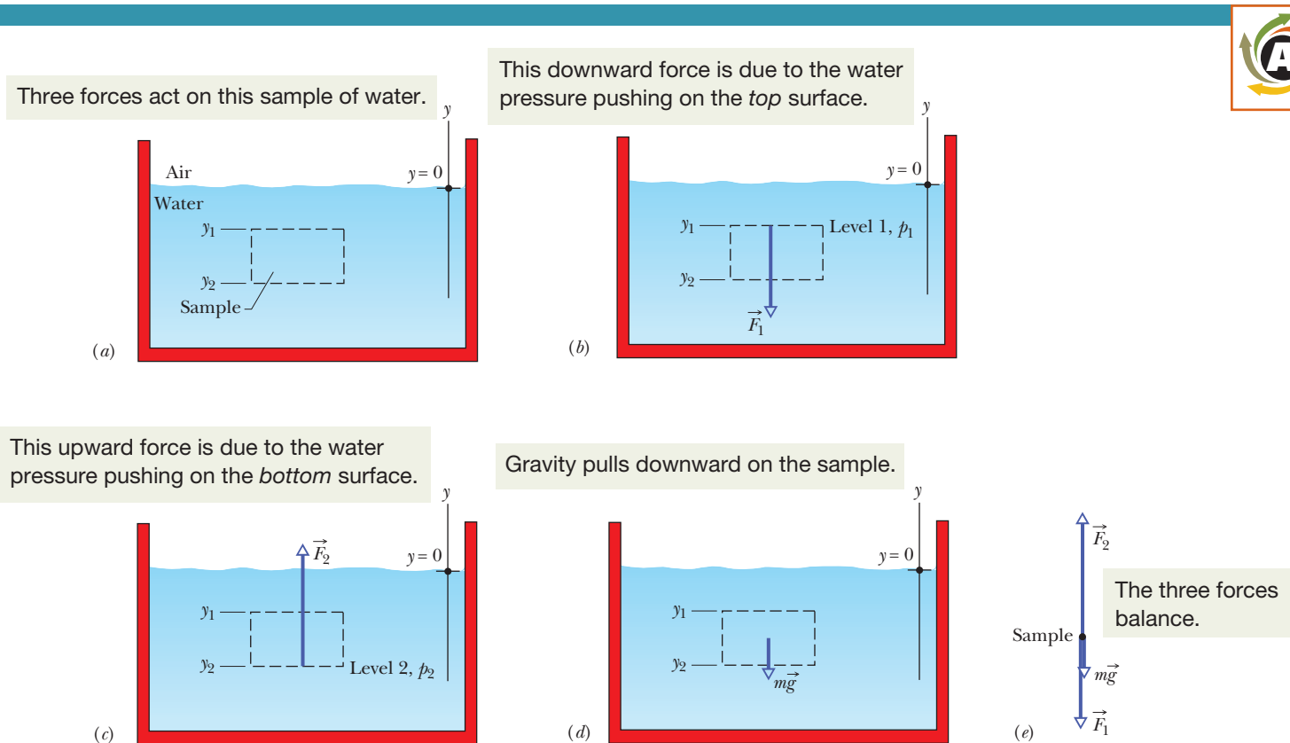
Figure 14-2 (a) A tank of water in which a sample of water is contained in an imaginary cylinder of horizontal base area A . (b)–(d) Force \vec{F}_1 acts at the top surface of the cylinder; force \vec{F}_2 acts at the bottom surface of the cylinder; the gravitational force on the water in the cylinder is represented by m\vec{g} . (e) A free-body diagram of the water sample. In WileyPLUS , this figure is available as an animation with voiceover.
