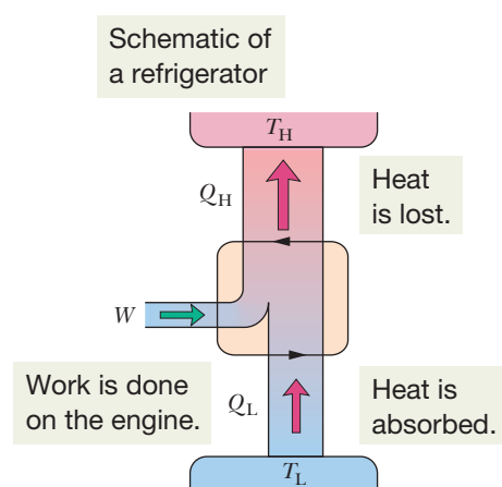
Figure 20-14 The elements of a Carnot refrigerator. The two black arrowheads on the central loop suggest the working substance operating in a cycle, as if on a p - V plot. Energy is transferred as heat Q_L to the working substance from the low-temperature reservoir. Energy is transferred as heat Q_H to the high-temperature reservoir from the working substance. Work W is done on the refrigerator (on the working substance) by something in the environment.
