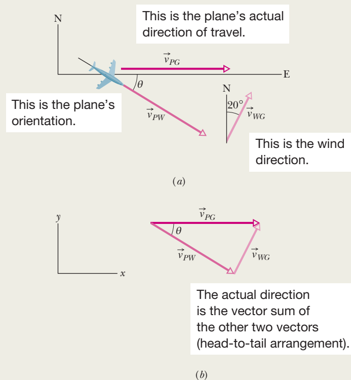
Figure 4-20 A plane flying in a wind.
