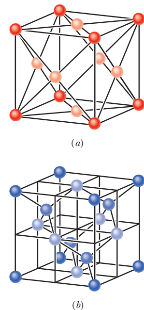
Figure 41-1 (a) The unit cell for copper is a cube. There is one copper atom (darker) at each corner of the cube and one copper atom (lighter) at the center of each face of the cube. The arrangement is called face-centered cubic . (b) The unit cell for either silicon or the carbon atoms in diamond is also a cube, the atoms being arranged in what is called a diamond lattice . There is one atom (darkest) at each corner of the cube and one atom (lightest) at the center of each cube face; in addition, four atoms (medium color) lie within the cube. Every atom is bonded to its four nearest neighbors by a two-electron covalent bond (only the four atoms within the cube show all four nearest neighbors).
