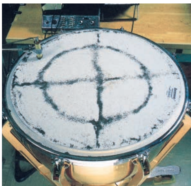
Figure 16-22 One of many possible standing wave patterns for a kettledrum head, made visible by dark powder sprinkled on the drumhead. As the head is set into oscillation at a single frequency by a mechanical oscillator at the upper left of the photograph, the powder collects at the nodes, which are circles and straight lines in this two-dimensional example.
