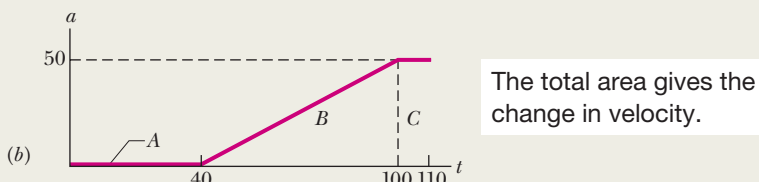
Figure 2-15 (a) The a(t) curve of the torso and head of a volunteer in a simulation of a rear-end collision. (b) Breaking up the region between the plotted curve and the time axis to calculate the area.
