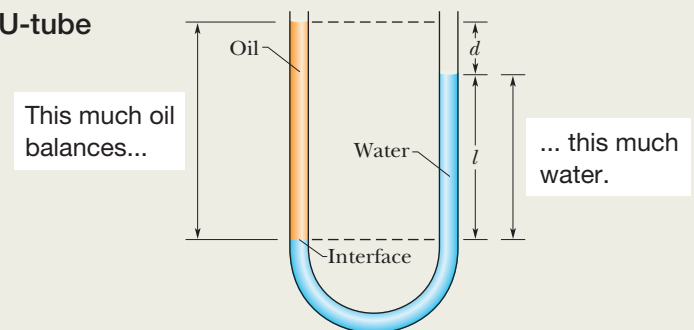
Figure 14-4 The oil in the left arm stands higher than the water.
