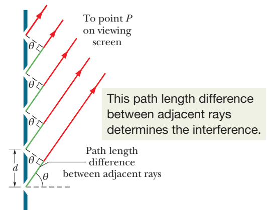
Figure 36-20 The rays from the rulings in a diffraction grating to a distant point P are approximately parallel. The path length difference between each two adjacent rays is d \sin \theta , where \theta is measured as shown. (The rulings extend into and out of the page.)
