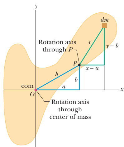
Figure 10-12 A rigid body in cross section, with its center of mass at O . The parallel-axis theorem (Eq. 10-36) relates the rotational inertia of the body about an axis through O to that about a parallel axis through a point such as P , a distance h from the body's center of mass.
