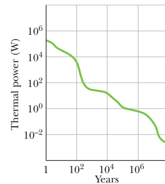
Figure 43-7 The thermal power released by the radioactive wastes from one year's operation of a typical large nuclear power plant, shown as a function of time. The curve is the superposition of the effects of many radionuclides, with a wide variety of half-lives. Note that both scales are logarithmic.
