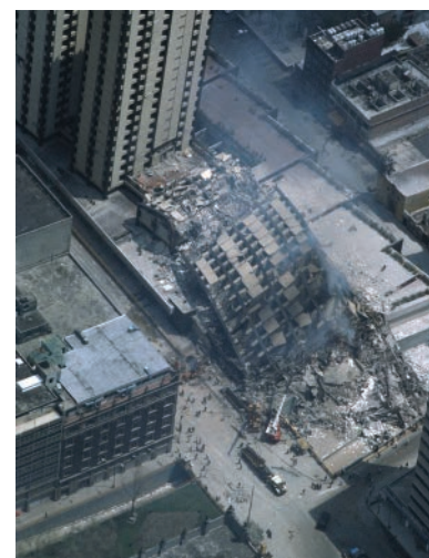
Figure 15-19 In 1985, buildings of intermediate height collapsed in Mexico City as a result of an earthquake far from the city. Taller and shorter buildings remained standing.
