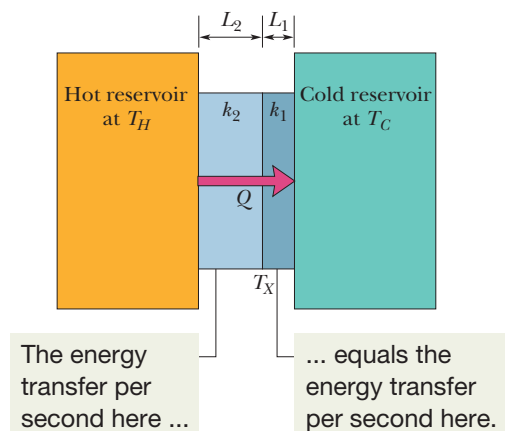
Figure 18-19 Heat is transferred at a steady rate through a composite slab made up of two different materials with different thicknesses and different thermal conductivities. The steady-state temperature at the interface of the two materials is T_X .
