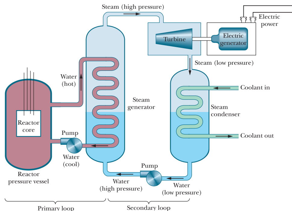
Figure 43-6 A simplified layout of a nuclear power plant, based on a pressurized-water reactor. Many features are omitted – among them the arrangement for cooling the reactor core in case of an emergency.
