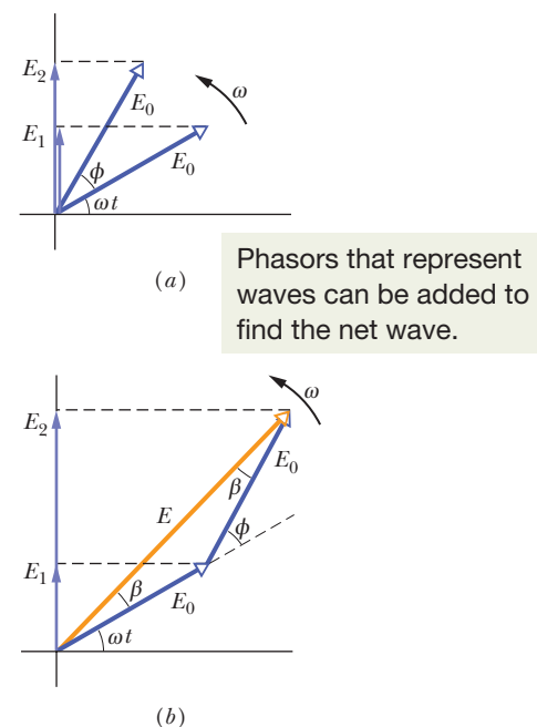
Figure 35-13 (a) Phasors representing, at time t , the electric field components given by Eqs. 35-20 and 35-21. Both phasors have magnitude E_0 and rotate with angular speed \omega . Their phase difference is \phi . (b) Vector addition of the two phasors gives the phasor representing the resultant wave, with amplitude E and phase constant \beta .
