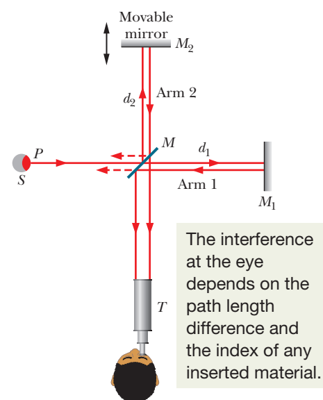
Figure 35-21 Michelson's interferometer, showing the path of light originating at point P of an extended source S . Mirror M splits the light into two beams, which reflect from mirrors M_1 and M_2 back to M and then to telescope T . In the telescope an observer sees a pattern of interference fringes.
