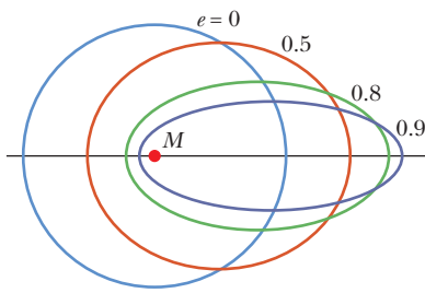
Figure 13-15 Four orbits with different eccentricities e about an object of mass M . All four orbits have the same semimajor axis a and thus correspond to the same total mechanical energy E .
