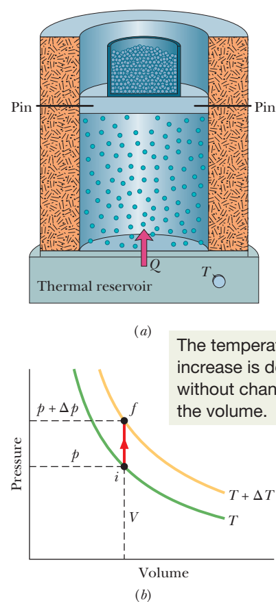
Figure 19-9 (a) The temperature of an ideal gas is raised from T to T + \Delta T in a constant-volume process. Heat is added, but no work is done. (b) The process on a p - V diagram.
