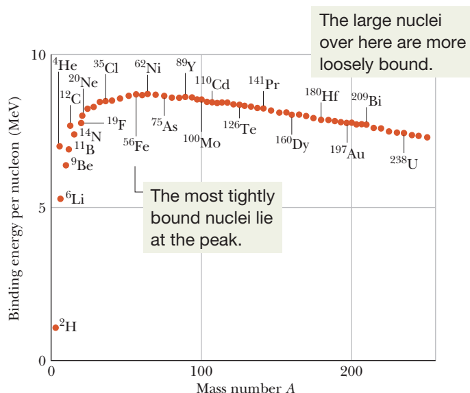
Figure 42-7 The binding energy per nucleon for some representative nuclides. The nickel nuclide ^{62}\text{Ni} has the highest binding energy per nucleon (about 8.794 60 MeV/nucleon) of any known stable nuclide. Note that the alpha particle ( ^4\text{He} ) has a higher binding energy per nucleon than its neighbors in the periodic table and thus is also particularly stable.
