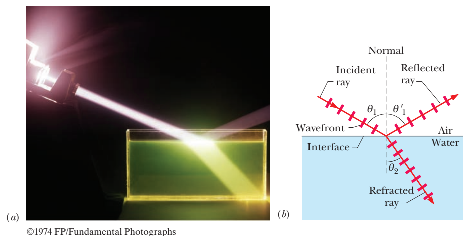
Figure 33-16 (a) A photograph showing an incident beam of light reflected and refracted by a horizontal water surface. (b) A ray representation of (a). The angles of incidence ( \theta_1 ), reflection ( \theta'_1 ), and refraction ( \theta_2 ) are marked.
