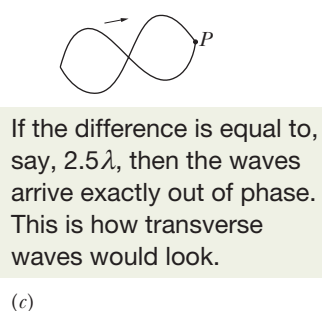
Figure 17-7 (a) Two point sources S_1 and S_2 emit spherical sound waves in phase. The rays indicate that the waves pass through a common point P . The waves (represented with transverse waves) arrive at P (b) exactly in phase and (c) exactly out of phase.
