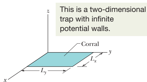
Figure 39-13 A rectangular corral — a two-dimensional version of the infinite potential well of Fig. 39-2 — with widths L_x and L_y .
