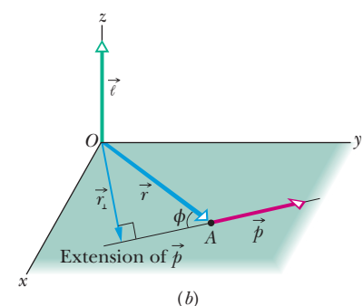
Figure 11-12 Defining angular momentum. A particle passing through point A has linear momentum \vec{p} (= m\vec{v}) with the vector \vec{p} lying in an xy plane. The particle has angular momentum \vec{\ell} (= \vec{r} \times \vec{p}) with respect to the origin O . By the right-hand rule, the angular momentum vector points in the positive direction of z . (a) The magnitude of \vec{\ell} is given by \ell = rp_{\perp} = rmv_{\perp} . (b) The magnitude of \vec{\ell} is also given by \ell = r_{\perp}p = r_{\perp}mv .
