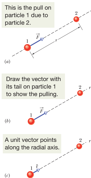
Figure 13-2 (a) The gravitational force \vec{F} on particle 1 due to particle 2 is an attractive force because particle 1 is attracted to particle 2. (b) Force \vec{F} is directed along a radial coordinate axis r extending from particle 1 through particle 2. (c) \vec{F} is in the direction of a unit vector \hat{r} along the r axis.
