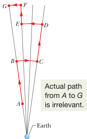
Figure 13-10 Near Earth, a baseball is moved from point A to point G along a path consisting of radial lengths and circular arcs.
