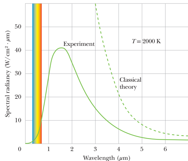
Figure 38-8 The solid curve shows the experimental spectral radiancy for a cavity at 2000 K. Note the failure of the classical theory, which is shown as a dashed curve. The range of visible wavelengths is indicated.
