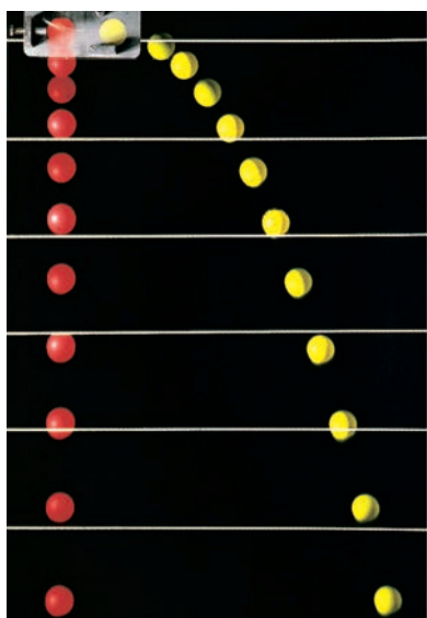
Figure 4-10 One ball is released from rest at the same instant that another ball is shot horizontally to the right. Their vertical motions are identical.
