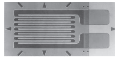
Figure 12-14 A strain gage of overall dimensions 9.8 mm by 4.6 mm. The gage is fastened with adhesive to the object whose strain is to be measured; it experiences the same strain as the object. The electrical resistance of the gage varies with the strain, permitting strains up to 3% to be measured.
