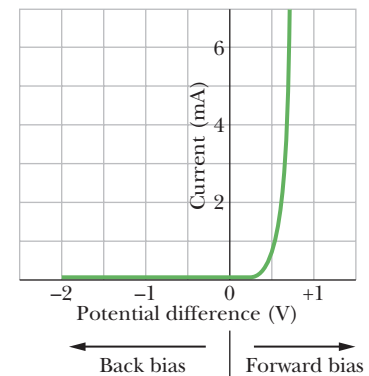
Figure 41-13 A current–voltage plot for a p - n junction, showing that the junction is highly conducting when forward-biased and essentially nonconducting when back-biased.
