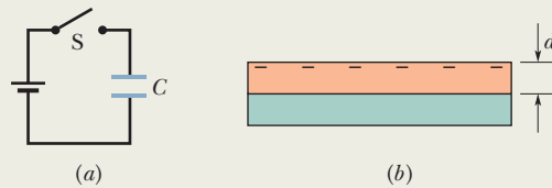
Figure 25-7 (a) A battery and capacitor circuit. (b) The lower capacitor plate.
